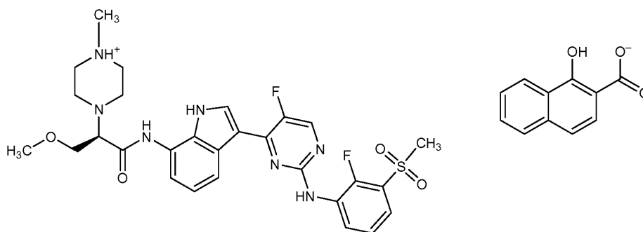
Formula (Ia)
