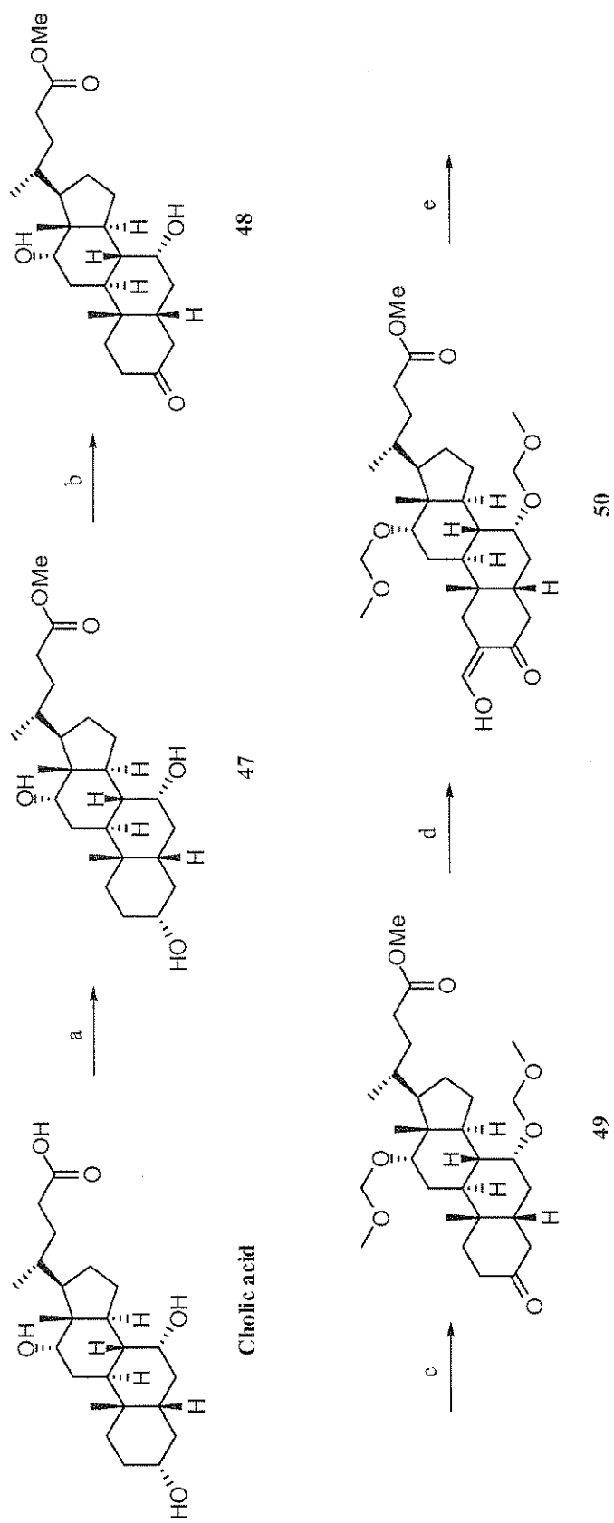
Scheme 13a:
