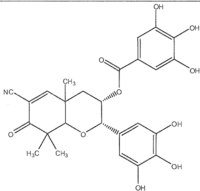
EGCG 1
