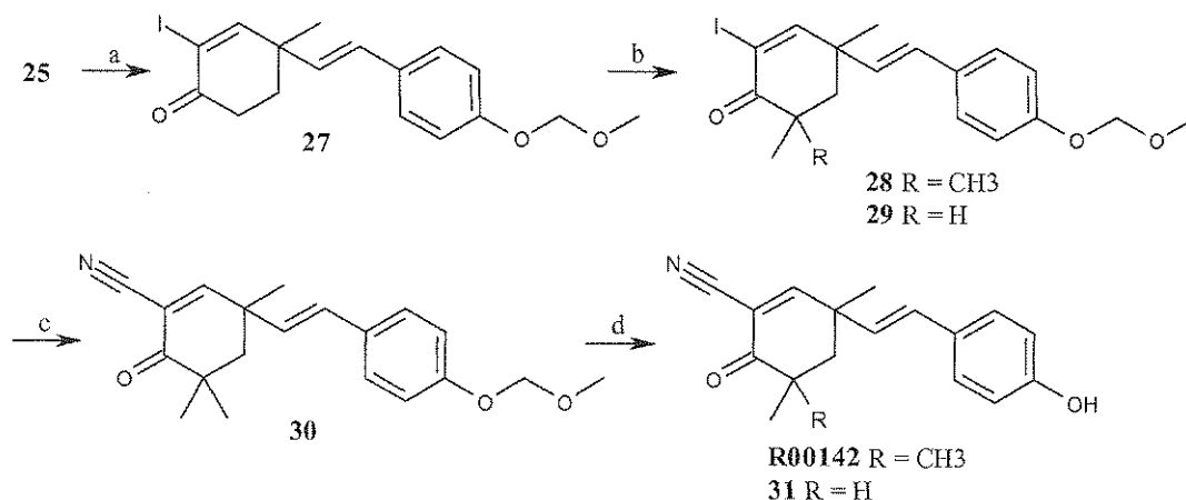
Scheme 6
