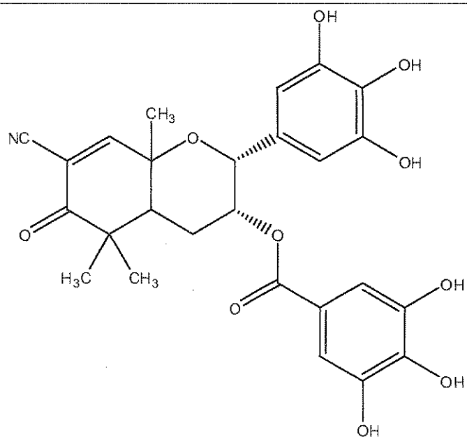
EGCG 2
