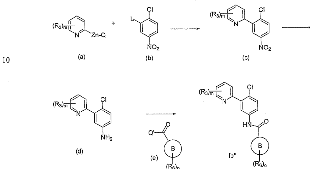
Scheme 8
