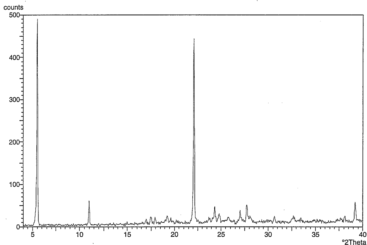
Figure E: XRPD pattern for N -benzyl-2-(benzylamino) ethanaminium salt of (2 S )-2-ethoxy-3- 15 (4-{2-[hexyl(2-phenylethyl)amino]-2-oxoethoxy}phenyl)propanoic acid
