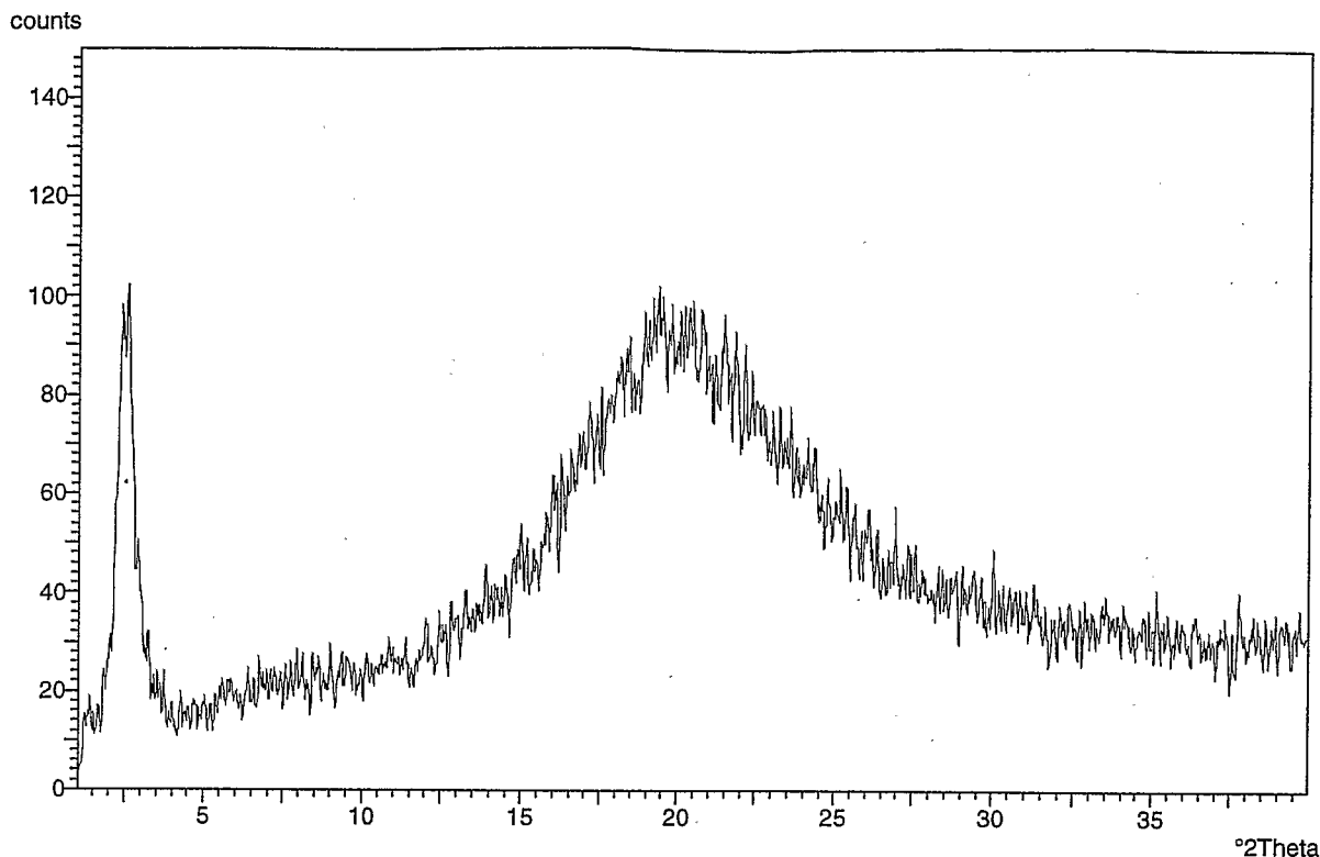
Figure B: XRPD pattern for L-arginine salt (2 S )-2-ethoxy-3-(4-{2-[hexyl(2-phenylethyl)amino]-2-oxoethoxy}phenyl)propanoic acid
