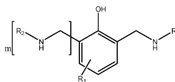
(Formula II)
