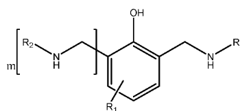
(Formula II)
