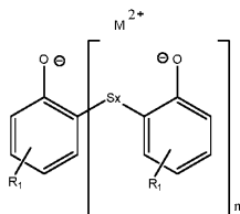
(Formula I)
