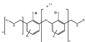
Formula Ib
