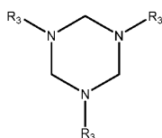
(Formula III)
