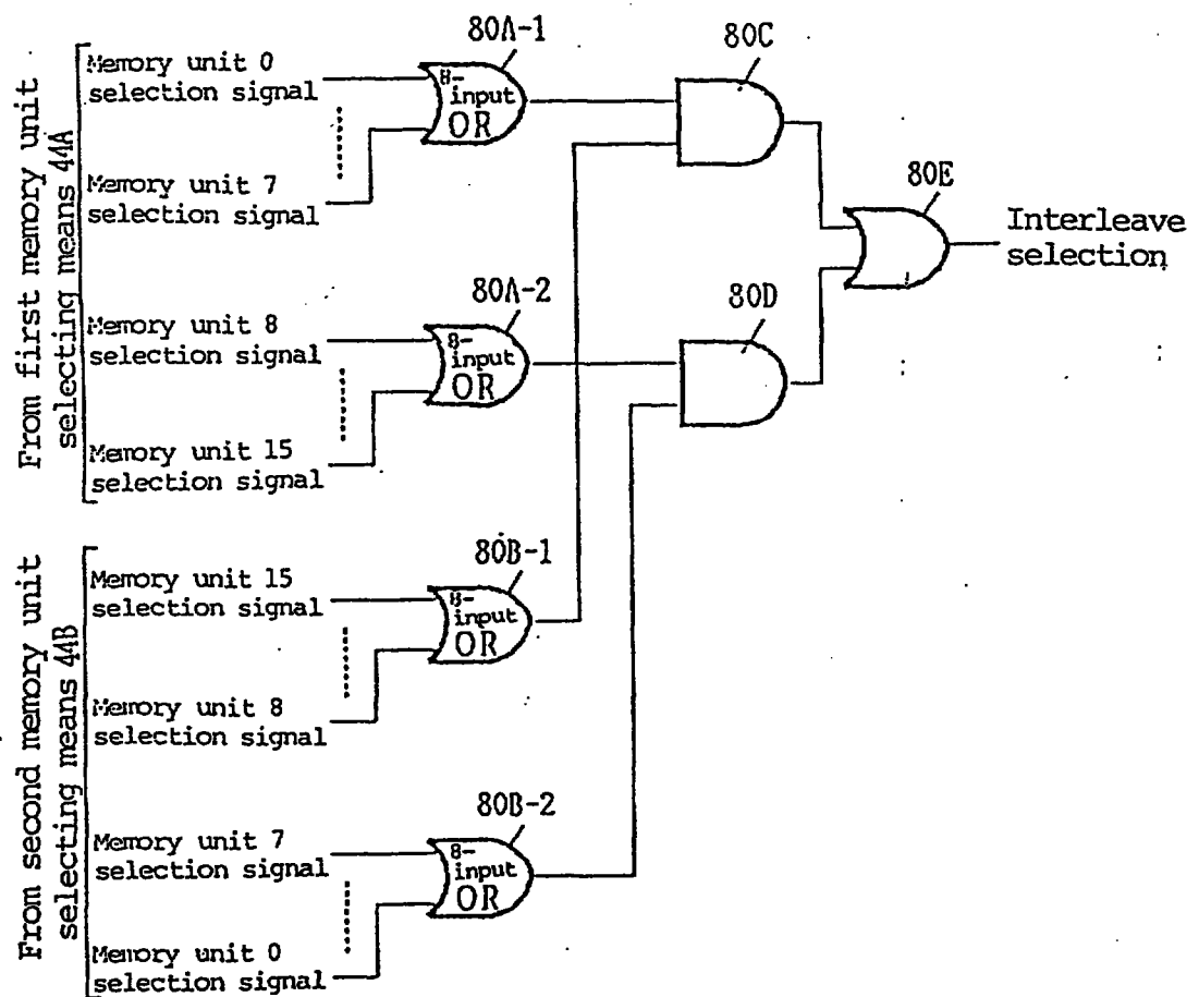
Interleave/non-interleave selecting circuit 80
