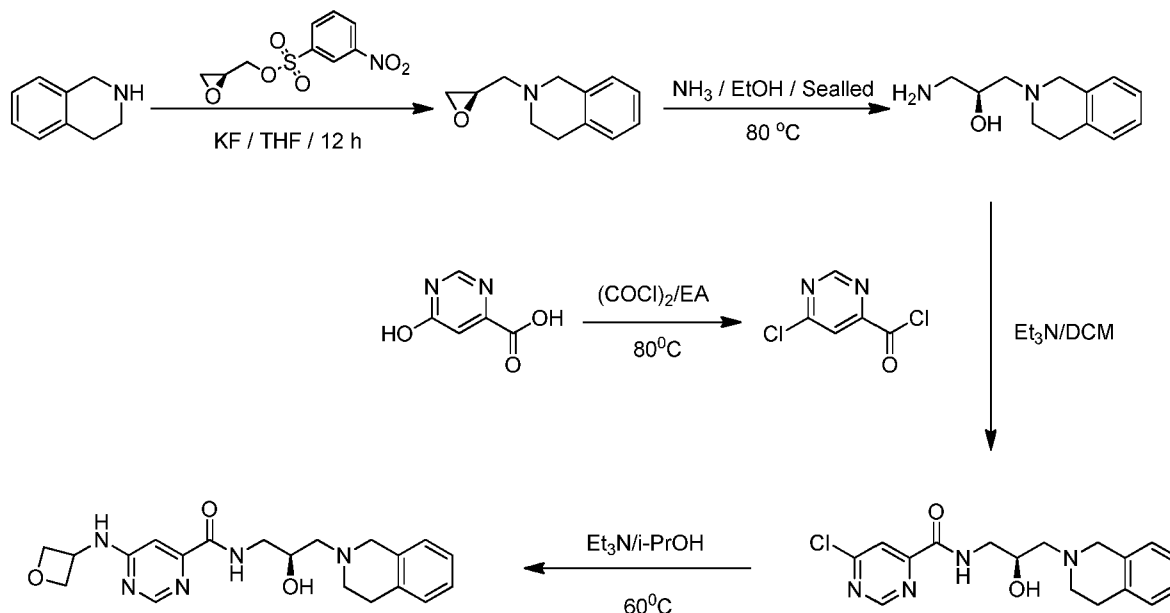
Scheme 7
