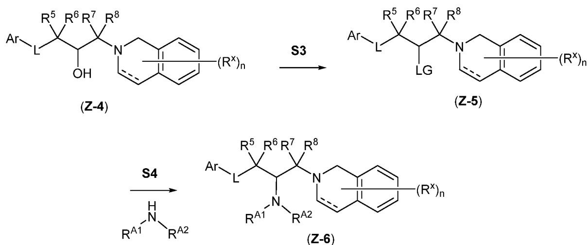
Scheme 5
