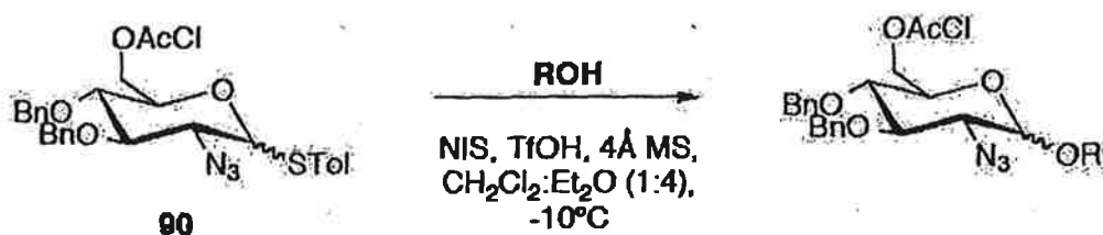
Scheme 5: Glycosylation reaction with the 2-azido-2-deoxythioglucoside donor 90 .
