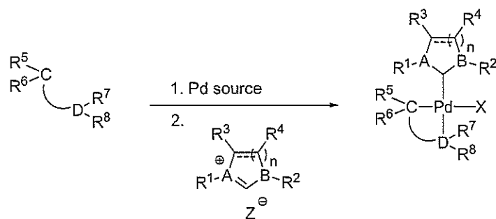
Scheme 1
