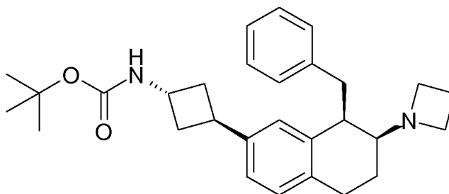
12.1 tert-Butyl ((1R,3r)-3-((7S,8R)-7-(azetidin-1-yl)-8-benzyl-5,6,7,8-tetrahydronaphthalen-2-yl)cyclobutyl)carbamate
