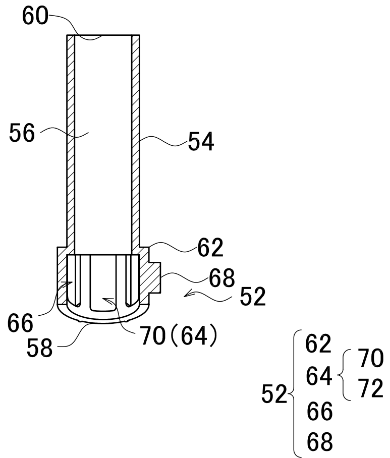
Sectional View IV-IV
