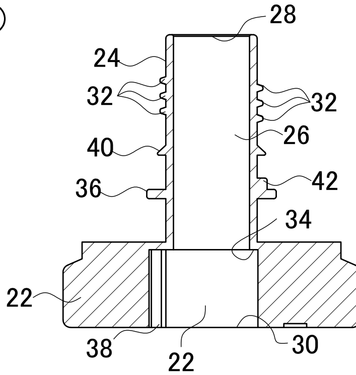
Sectional View III-III
