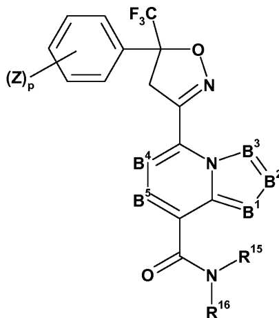
Formula (III)
