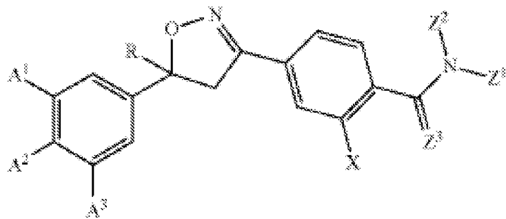
Formula (II)
