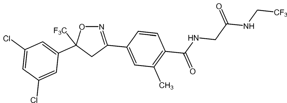
Compound B
