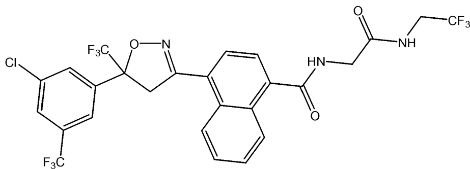
Compound A
