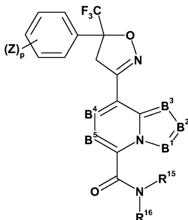
Formula (IV)
