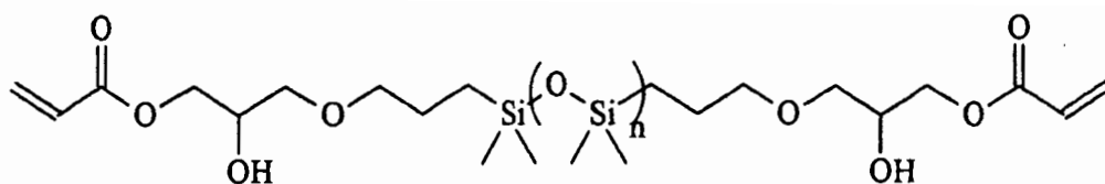
TRIS2-HOEOP2
