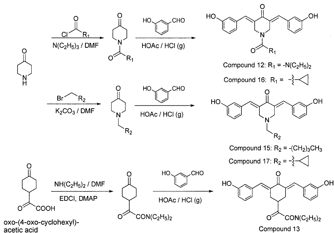
Scheme 6
