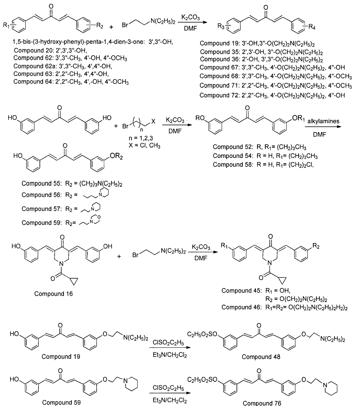
Scheme 8
