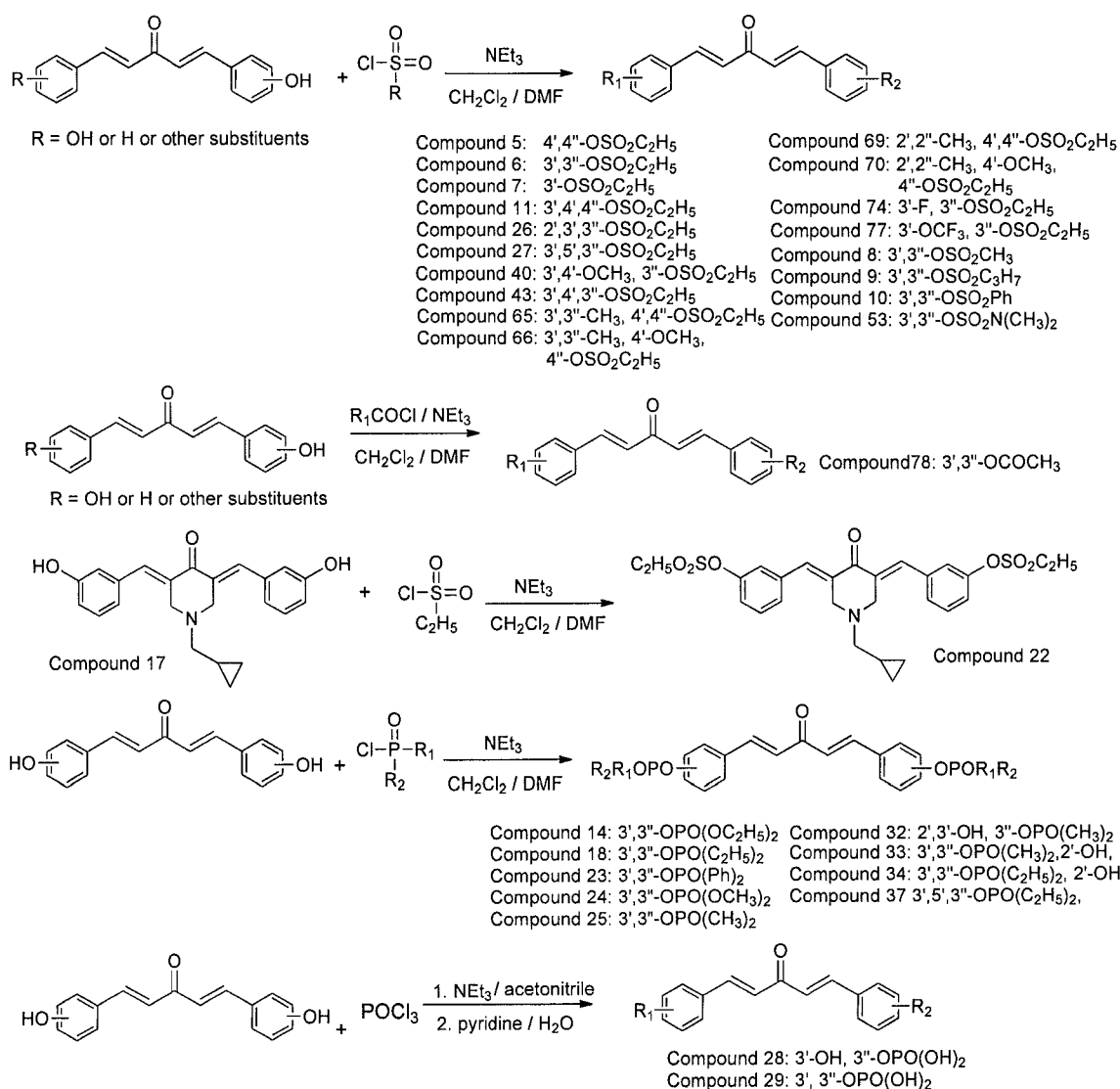
Scheme 7
