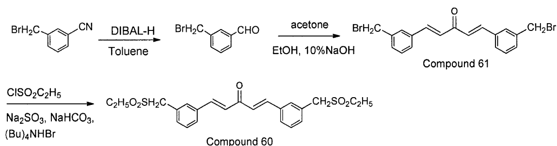
Scheme 10
