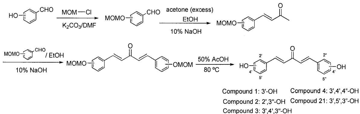
Scheme 4
