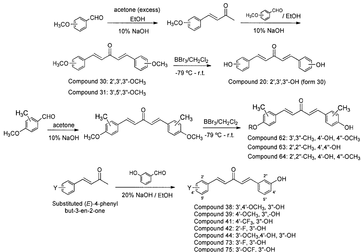
Scheme 5
