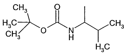
N-BOC-valyl
