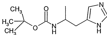
N-BOC-histidinyl
