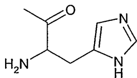
histidinyl
