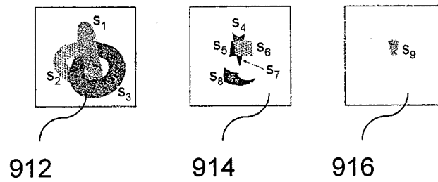
Region Labeling
