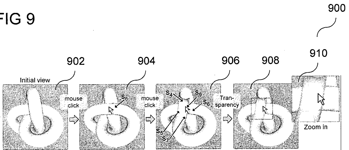
Region Labeling
