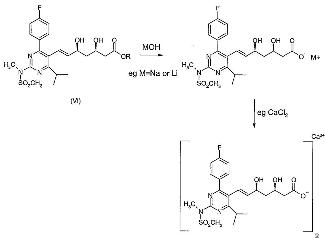
Scheme 2
