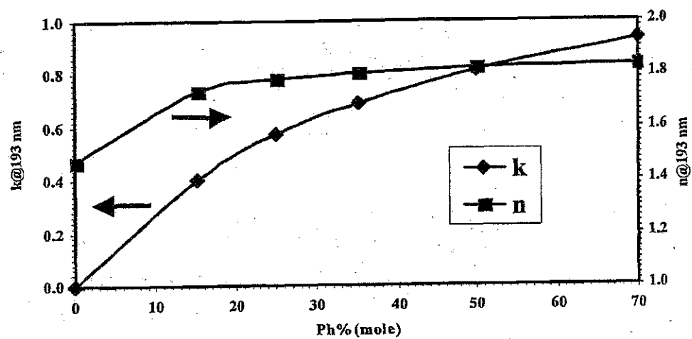
Dependence of Ph% on k@193\text{nm} of T(Ph)T(H) Resin
