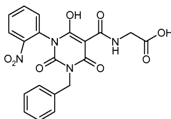
N -{[6-Hydroxy-1-(2-nitrophenyl)-2,4-dioxo-3-(phenylmethyl)-1,2,3,4-tetrahydro-5-pyrimidinyl]carbonyl}glycine
