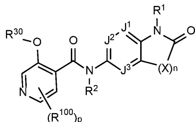
Formula I-1-B
