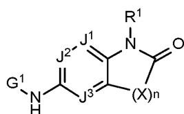
Formula III-1
