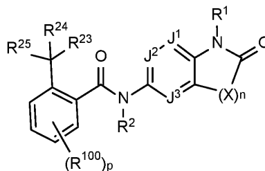
Formula I-2-A,
