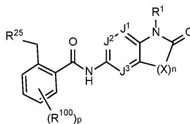
Formula I-2-A1,
