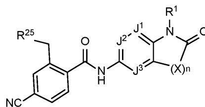
Formula I-2-A3
