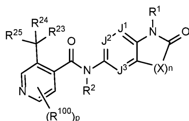
Formula I-1-A,
