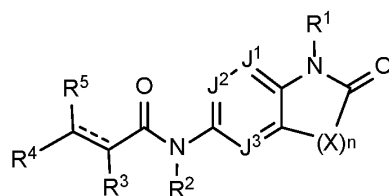
Formula I-O,
