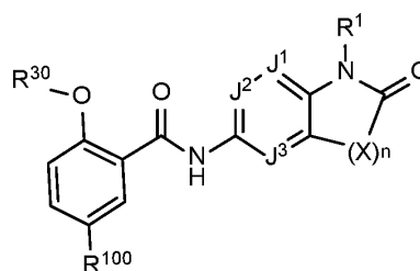
Formula I-2-B1,
