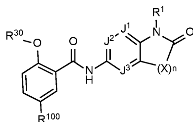
Formula I-2-B1,
