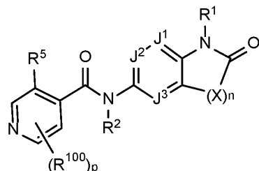
Formula I-1,
