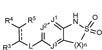
Formula II-3
