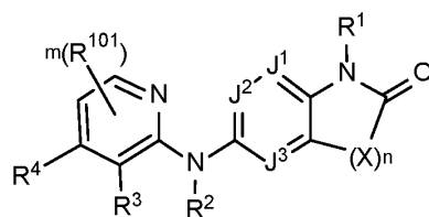
Formula I-F,
