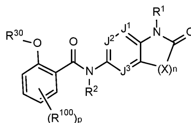
Formula I-2-B,
