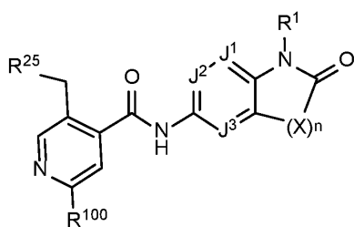
Formula I-1-A2
