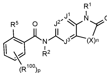
Formula I-2,
