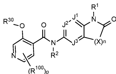
Formula I-1-B
