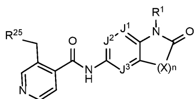
Formula I-1-A3
