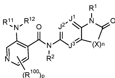
Formula I-1-C
