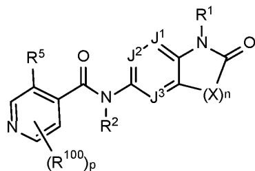
Formula I-1,
