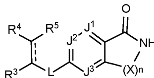
Formula II-2
