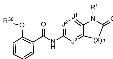
Formula I-2-B2,
