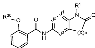
Formula I-2-B2,
