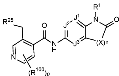
Formula I-1-A1
