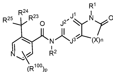
Formula I-1-A,
