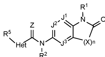
Formula I-P,
