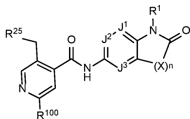
Formula I-1-A2
