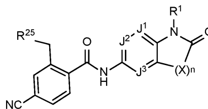
Formula I-2-A3
