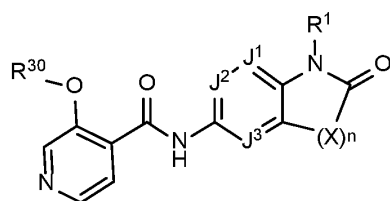
Formula I-1-B2
