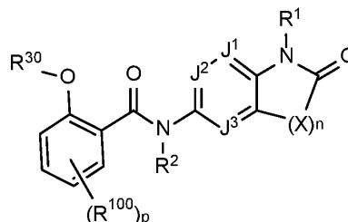
Formula I-2-B,
