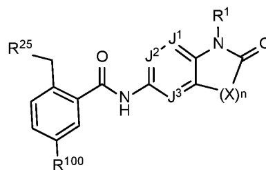
Formula I-2-A2,
