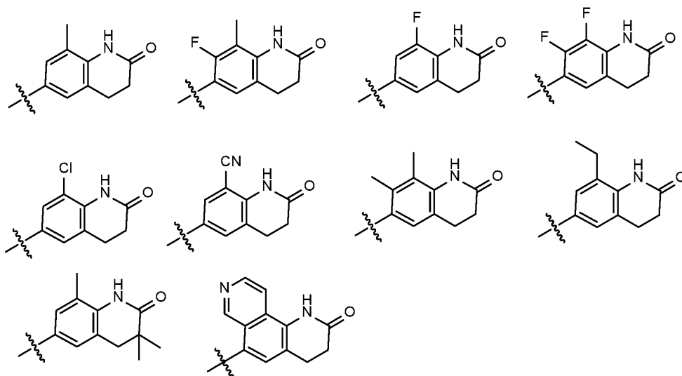
Formula III
