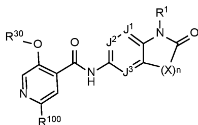
Formula I-1-B1
