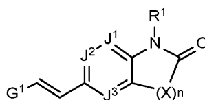
Formula III-2
