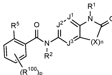
Formula I-2,
