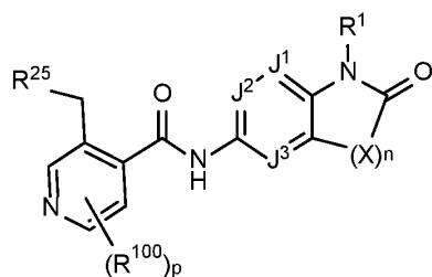
Formula I-1-A1
