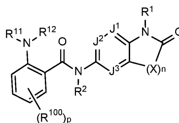
Formula I-2-C,
