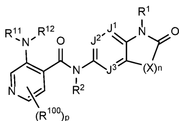
Formula I-1-C
