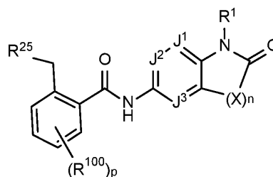
Formula I-2-A1,
