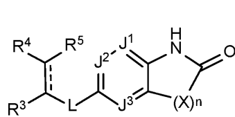
Formula II-1
