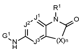
Formula III-1
