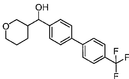
diastereomer A
