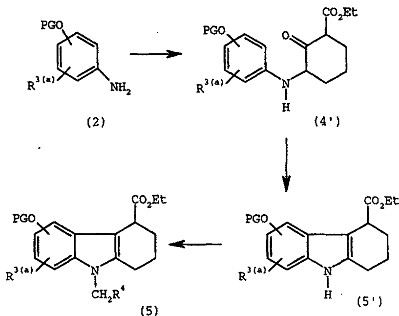
Scheme I(b)
