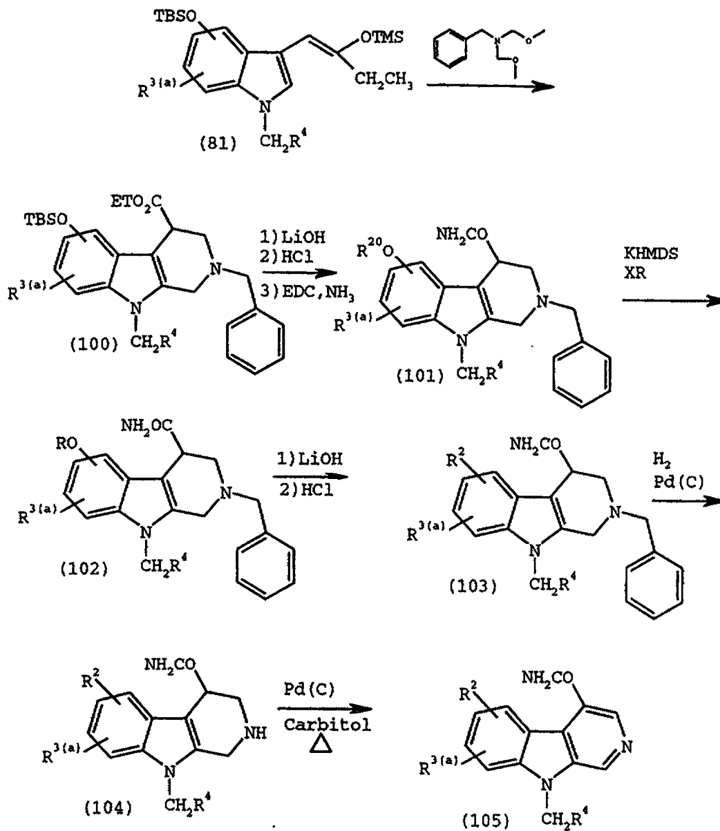
Scheme V(b)
