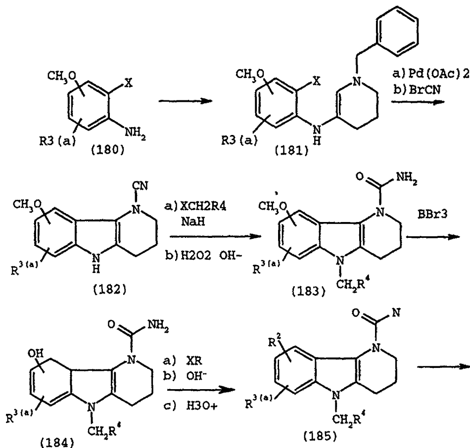
Scheme V(a)
