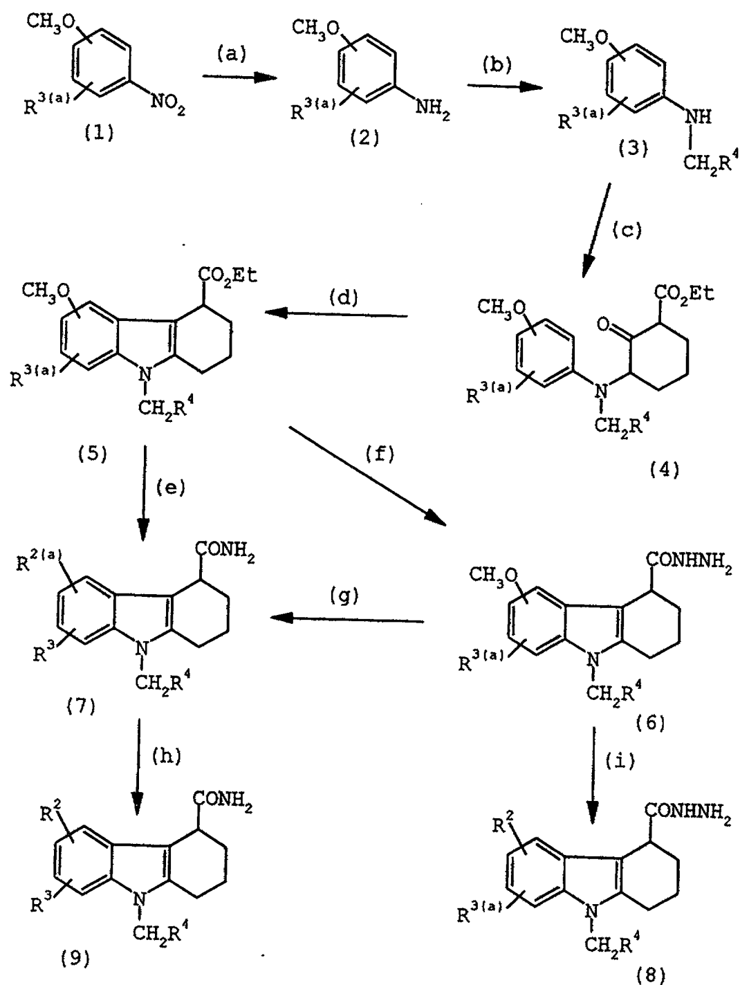
Scheme I (a)
