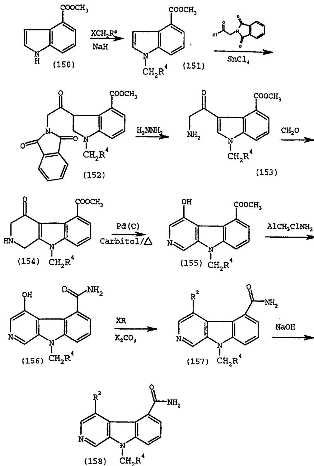
Scheme VIII(a)
