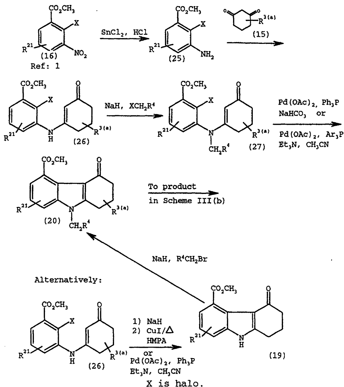
Scheme III(c)
