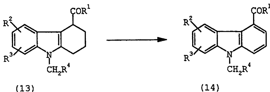
Scheme III (a)
