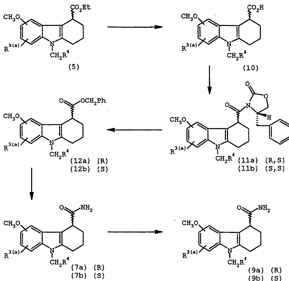
Scheme II
