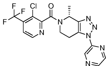
Example 341: (R*)-(3-chloro-4-(trifluoromethyl)pyridin-2-yl)(4-methyl-1-(pyrazin-2-yl)-6,7-dihydro-1H-[1,2,3]triazolo[4,5-c]pyridin-5(4H)-yl)methanone
