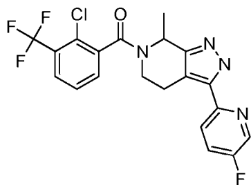
Example 431: (2,3-dichlorophenyl)(7-methyl-3-(pyrimidin-2-yl)-4,5-dihydro-2H-pyrazolo[3,4-c]pyridin-6(7H)-yl)methanone.
