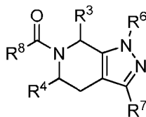
Formula (IIa)
