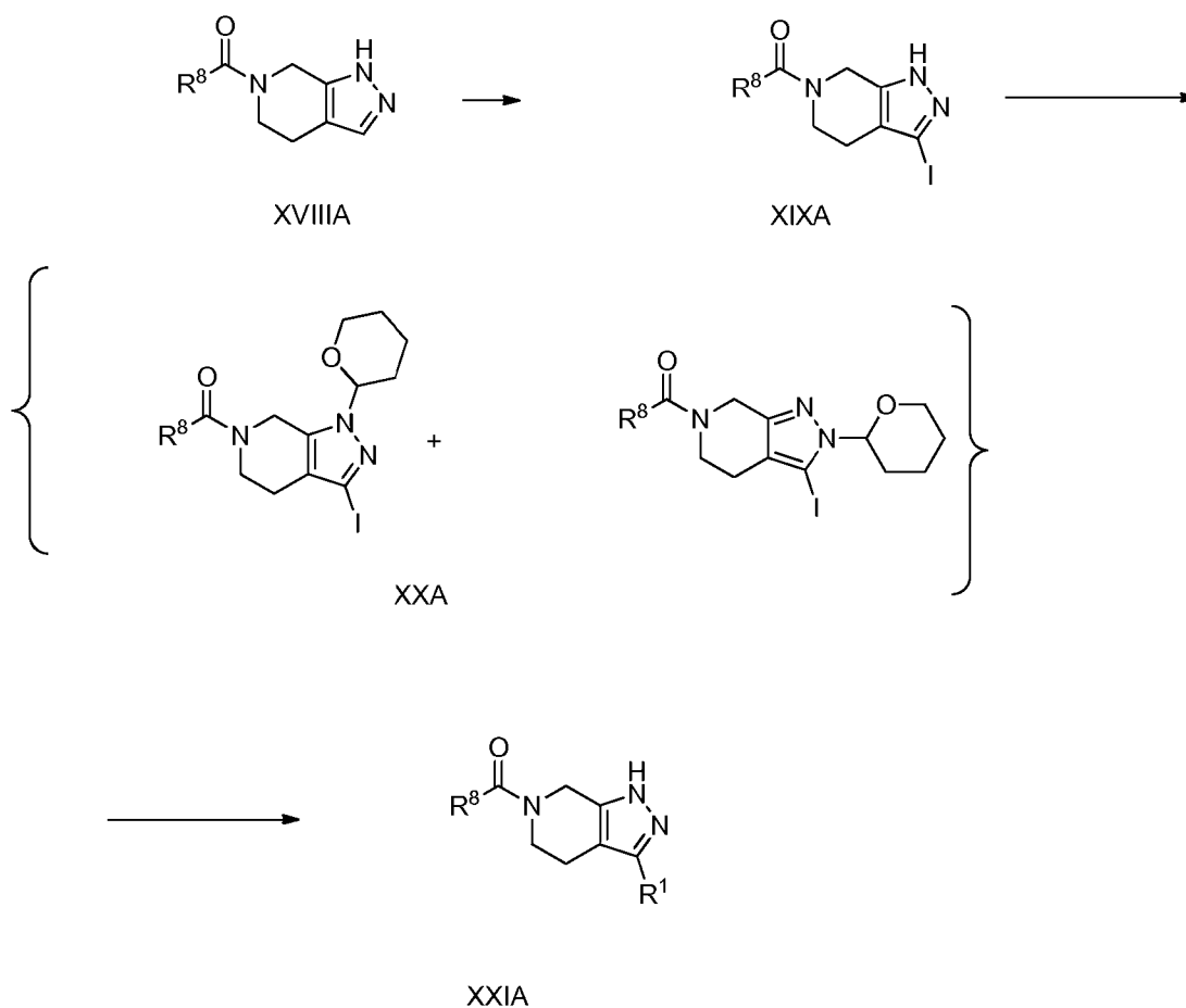
Scheme 6
