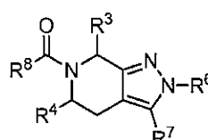
Formula (IIb)
