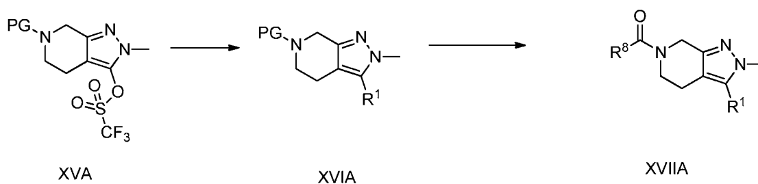
Scheme 5
