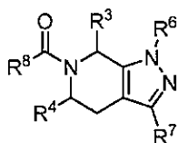
Formula (IIa)
