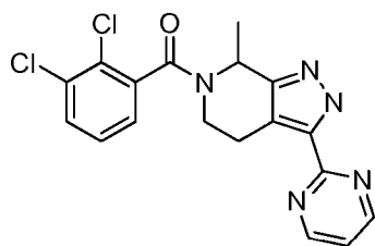
Example 431: (2,3-dichlorophenyl)(7-methyl-3-(pyrimidin-2-yl)-4,5-dihydro-2H-pyrazolo[3,4-c]pyridin-6(7H)-yl)methanone.
