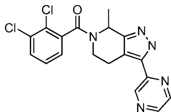
Example 433: (2,3-dichlorophenyl)(7-methyl-3-(pyrazin-2-yl)-4,5-dihydro-2H-pyrazolo[3,4-c]pyridin-6(7H)-yl)methanone.
