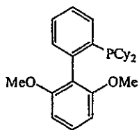
S Phos
