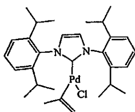
Carbene
