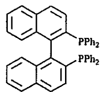
Rac-BINAP
