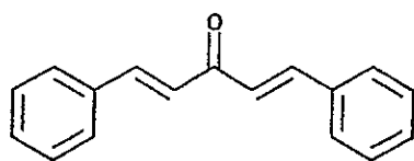
dba (dibenzylideneacetone)
