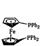
DPPF
