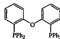
DPE-PHOS
