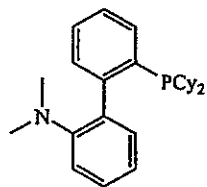
Cycloh_B
