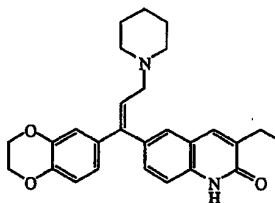
intermediate 41 (E isomer)
