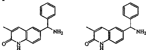
intermediate 17 and .HCl (1:1) intermediate 18
