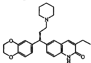
intermediate 40 (mixture of E + Z isomers)
