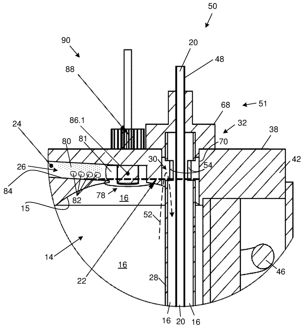
DETAIL H
