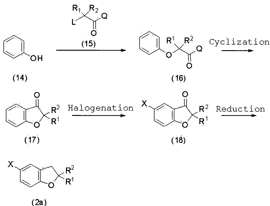
Reaction scheme 9
