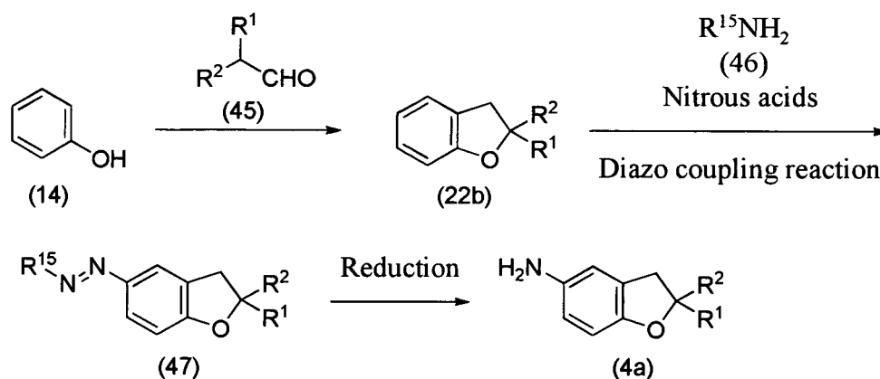
Reaction scheme 23
