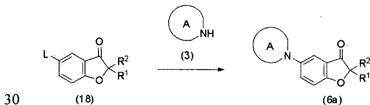
Reaction scheme 16
