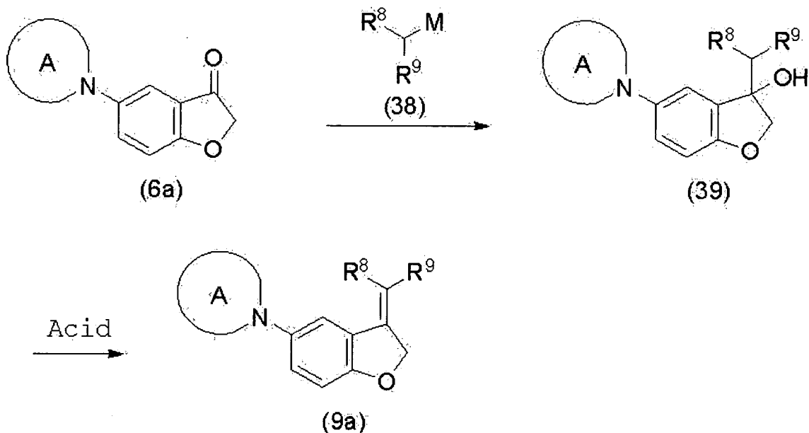
Reaction scheme 20
