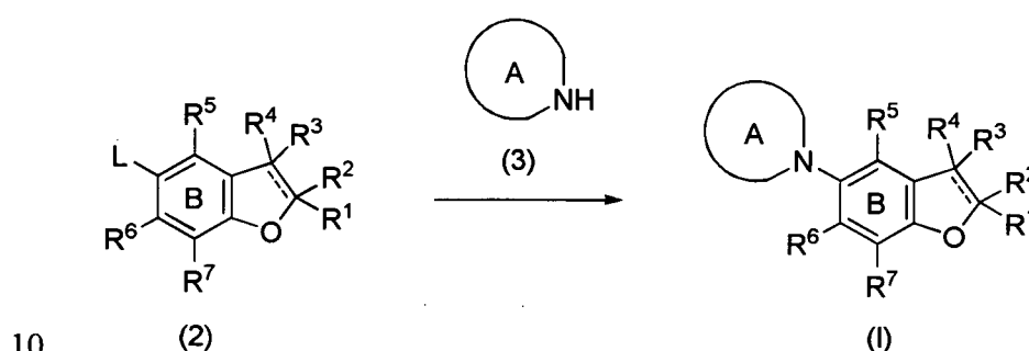
Reaction scheme 1:
