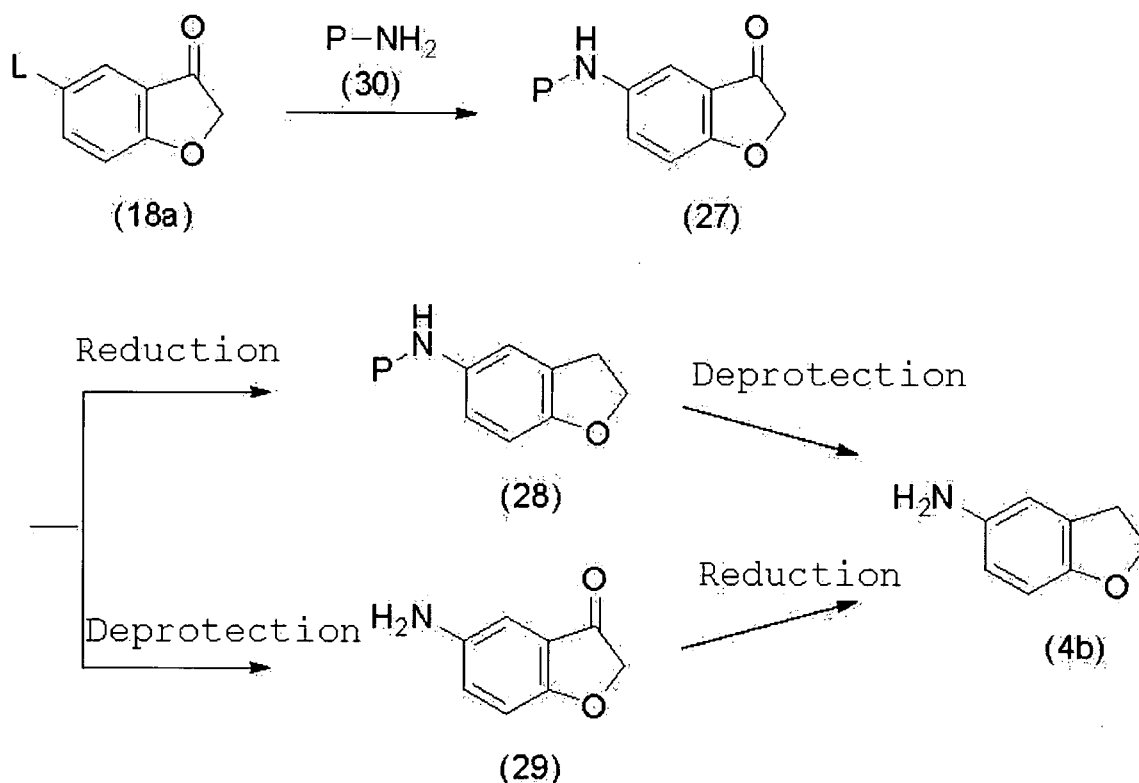
Reaction scheme 13
