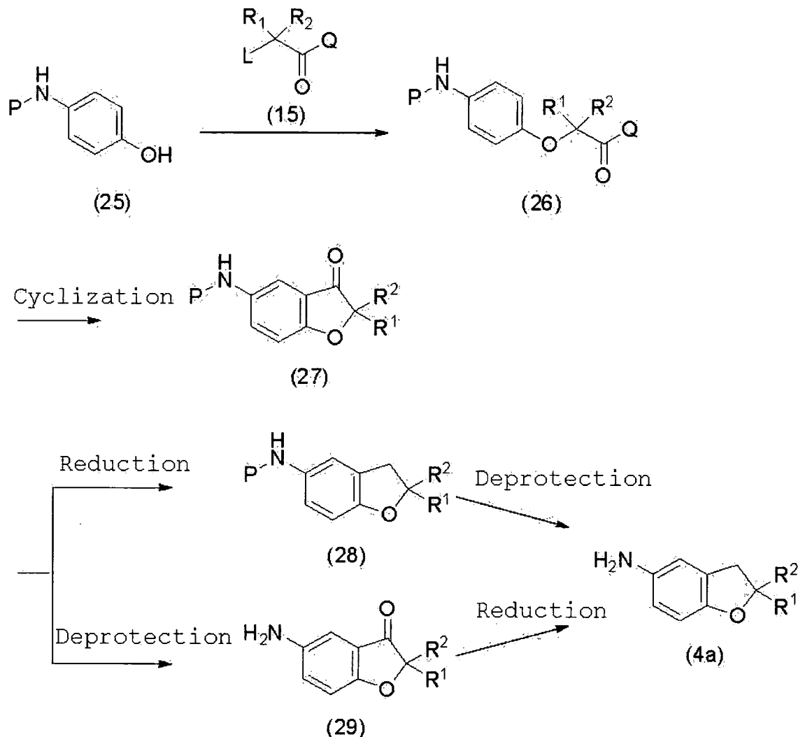
Reaction scheme 12
