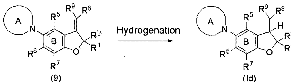
Reaction scheme 6
