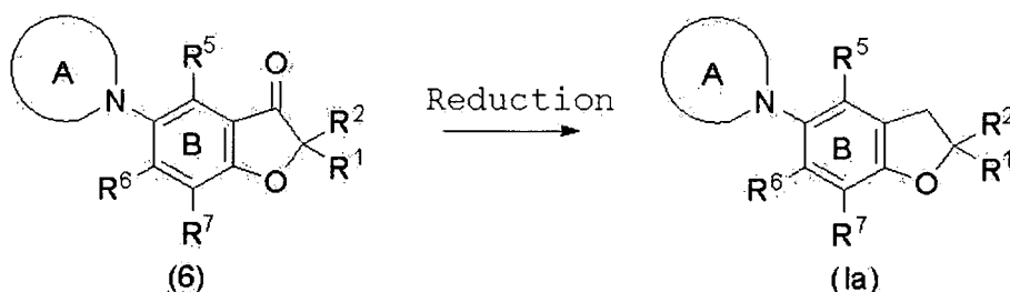
Reaction scheme 3
