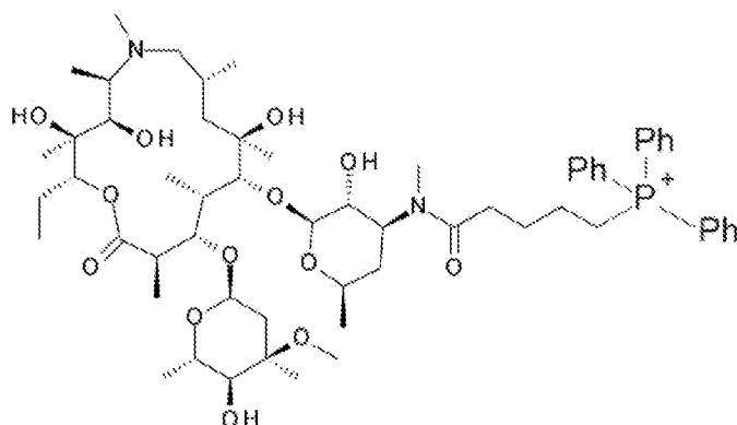
Tigecycline-TPP Conjugate
