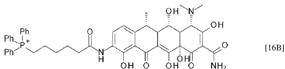
Doxycycline-TPP Conjugate
