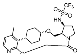
(Compound 94)
