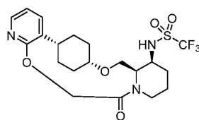
(Compound 91)
