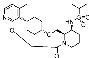
(Compound 10)
