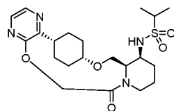
(Compound 66)
