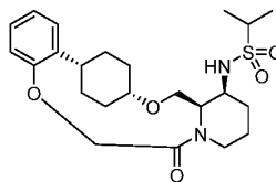
(Compound 3)
