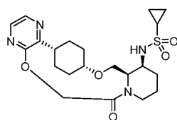
(Compound 65)
