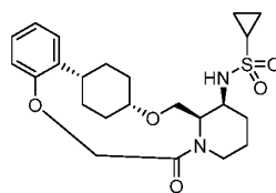
(Compound 1)
