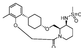
(Compound 37)
