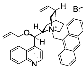
(-)-O-(9)-allyl-N-(9-anthracenylmethyl)cinchonidinium bromide
