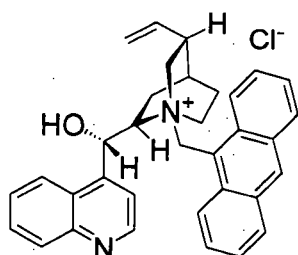
N-(9-anthracenylmethyl)cinchoninium chloride
