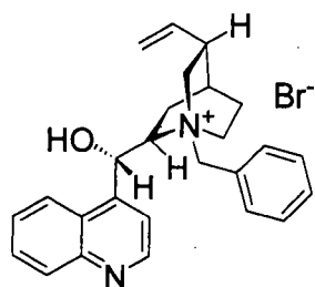
N-benzylcinchoninium bromide
