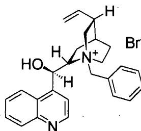
N-benzylcinchonidinium bromide
