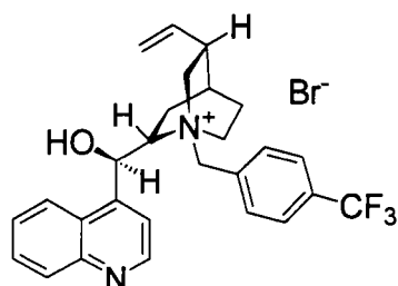
N-(4-trifluoromethylbenzyl)cinchonidinium bromide
