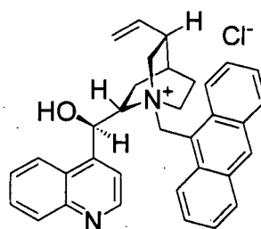
N-(9-anthracenylmethyl)cinchonidinium chloride
