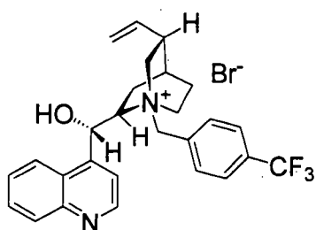
N-(4-trifluoromethylbenzyl)cinchoninium bromide
