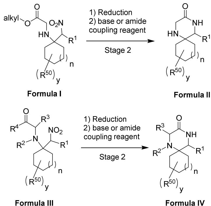
Scheme 11. Synthesis of Compounds of Formula II and Formula IV.
