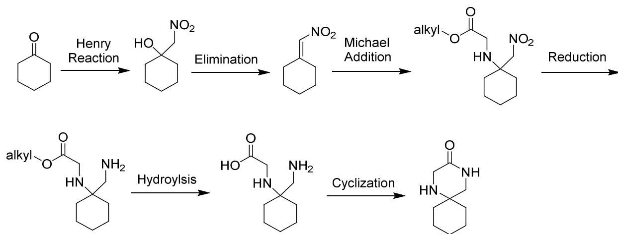
Scheme 3. Improved synthetic route to prepare 1,4-diazaspiro[5.5]undecan-3-one.
