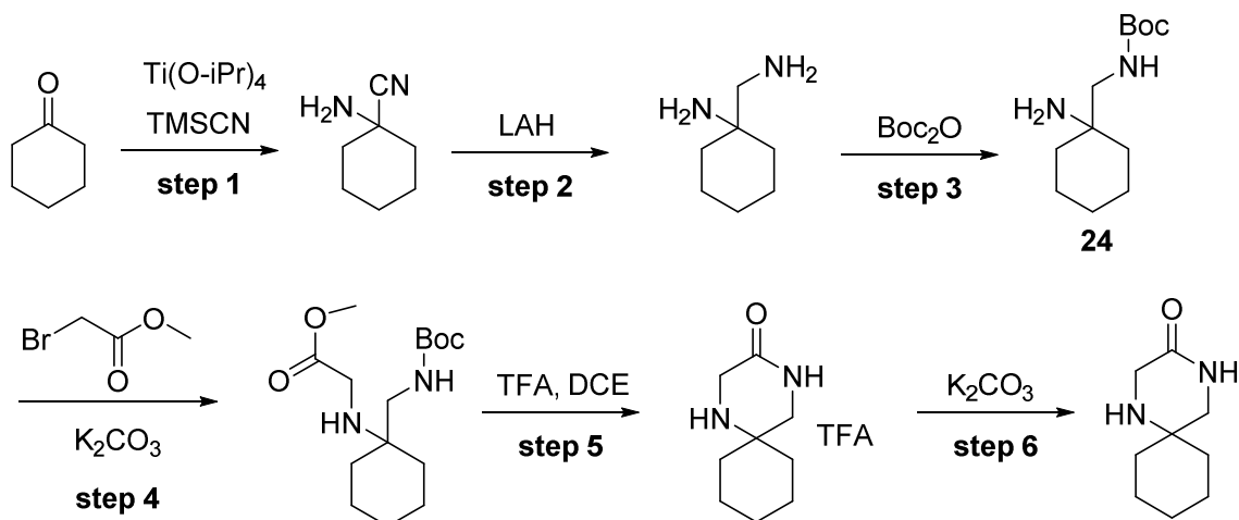
Scheme 2. Prior synthesis of 1,4-diazaspiro[5.5]undecan-3-one.
