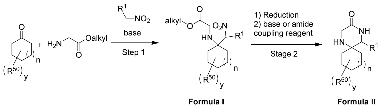
Scheme 7. General preparation of 1,4-diazaspiro[5.5]undecan-3-one with only two isolation steps.
