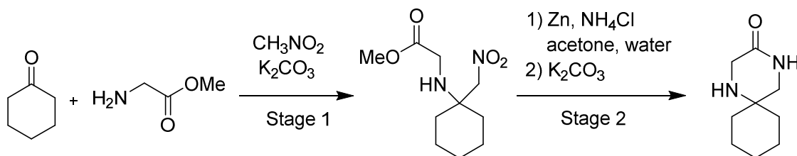
Scheme 4. Preparation of 1,4-diazaspiro[5.5]undecan-3-one with only two isolations.
