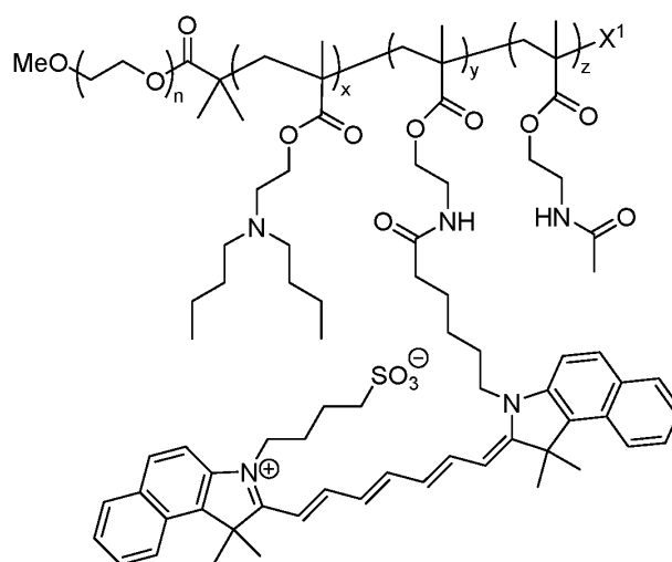
Formula (II-a).
