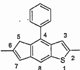
2,6-Dimethyl-4-phenyl-5 H - 1-thia-s-indacene
