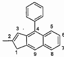
2-Methyl-4-phenyl-1 H -cyclo- penta[ b ]naphthalene
