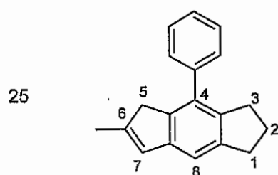
6-Methyl-4-phenyl-1,2,3,5- tetrahydro-s-indacene
