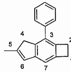
5-Methyl-3-phenyl-2,4-dihydro- 1 H -cyclobuta[ f ]indene
