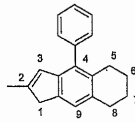
2-Methyl-4-phenyl-5,6,7,8- tetrahydro-1 H -cyclopenta- [ b ]naphthalene
