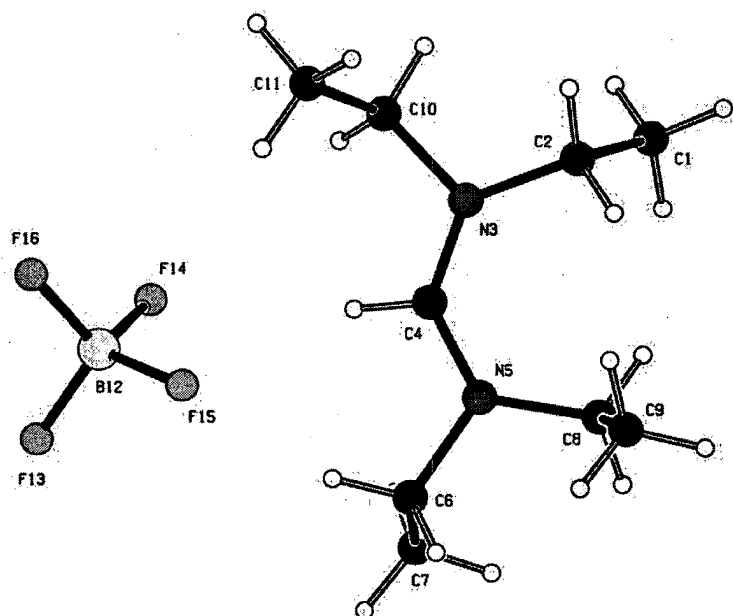
Figure 2: N,N,N',N'-Tetraethylformamidinium tetrafluoroborate
