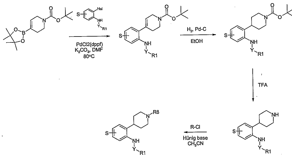
Scheme 10:
