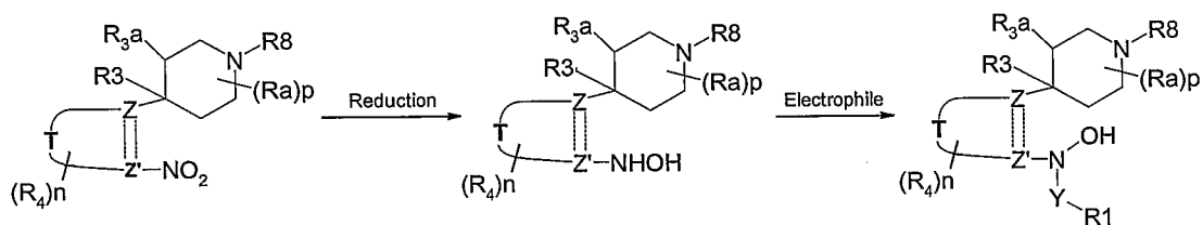
Scheme 7
