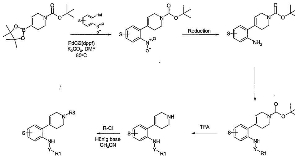
Scheme 11:
