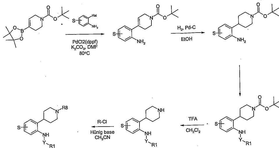
Scheme 10:
