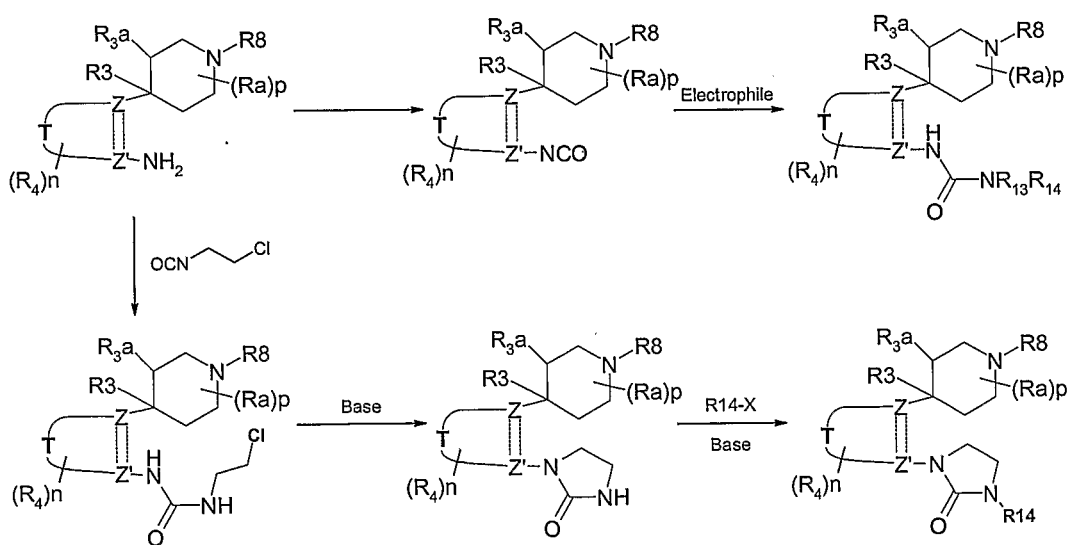
Scheme 7
