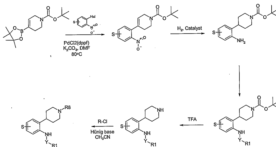
Scheme 8:
