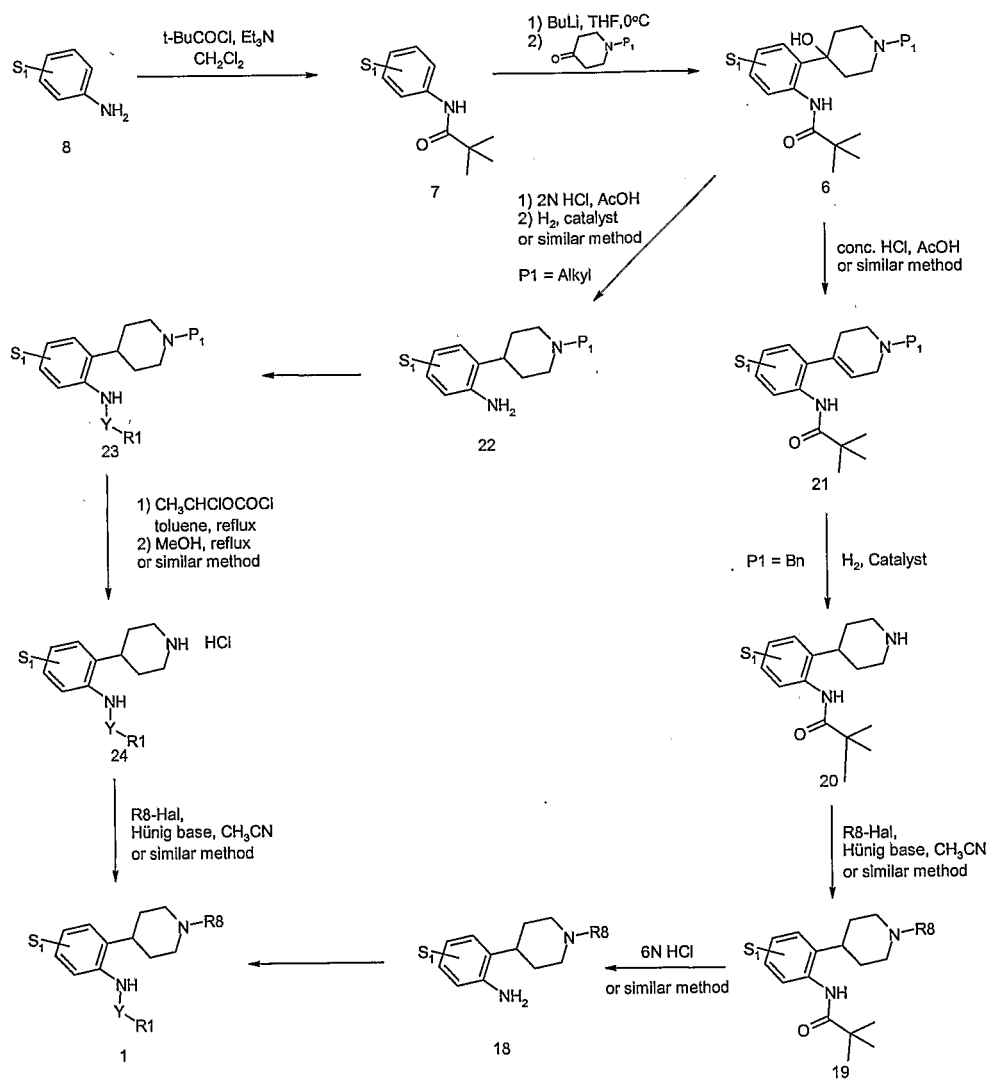
Scheme 3
