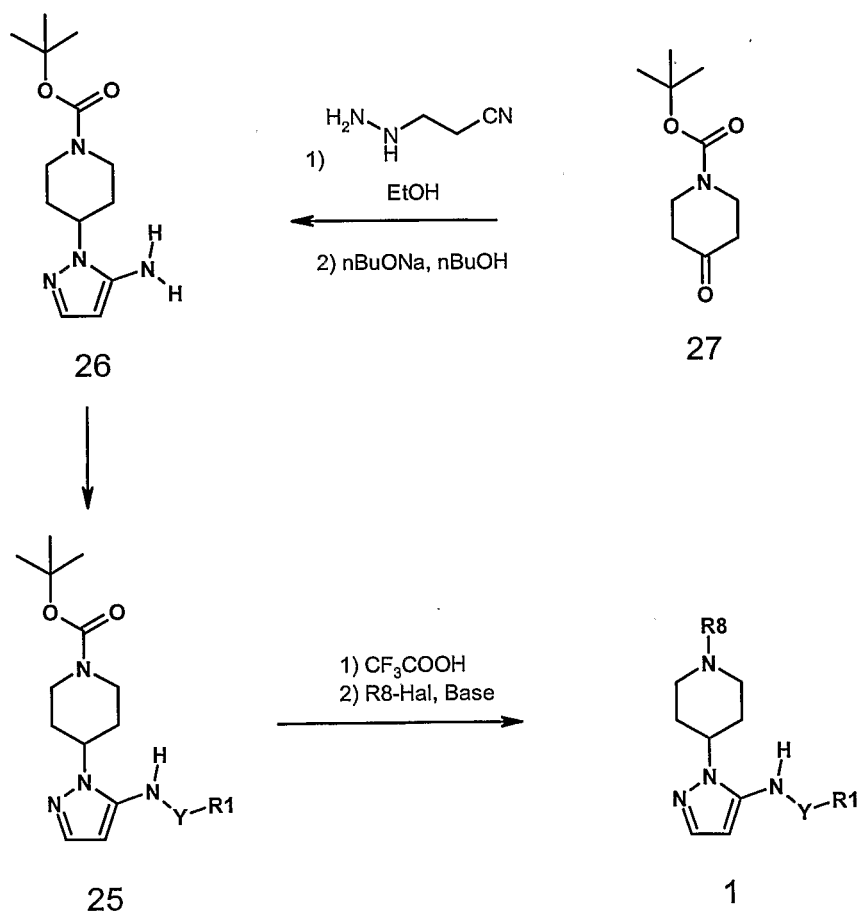
Scheme 4
