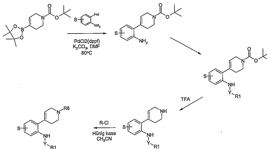
Scheme 13:
