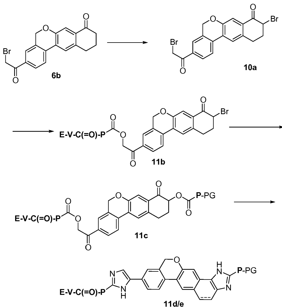
Scheme 11. Representative synthesis of E-V-C(=O)-P-W-P-R
