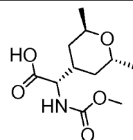
(S)-2-((2R,6R)-2,6-dimethyltetrahydro-2H-pyran-4-yl)-2-(methoxycarbonylamino)acetic acid
