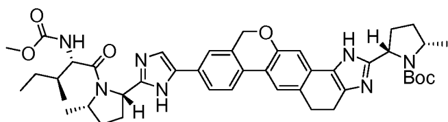
tert-butyl (2S,5S)-2-[9-(2-((2S,5S)-1-[N-(methoxycarbonyl)-L-isoleucyl]-5-methylpyrrolidin-2-yl)-1H-imidazol-5-yl)-1,4,5,11-tetrahydroisochromeno[4',3':6,7]naphtho[1,2-d]imidazol-2-yl]-5-methylpyrrolidine-1-carboxylate
