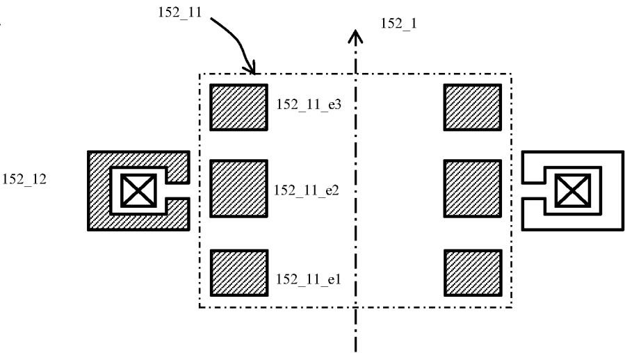
Figure 6B (Invention)
