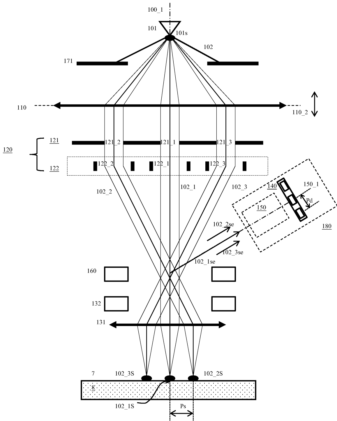
Figure 1 (Prior Art)
