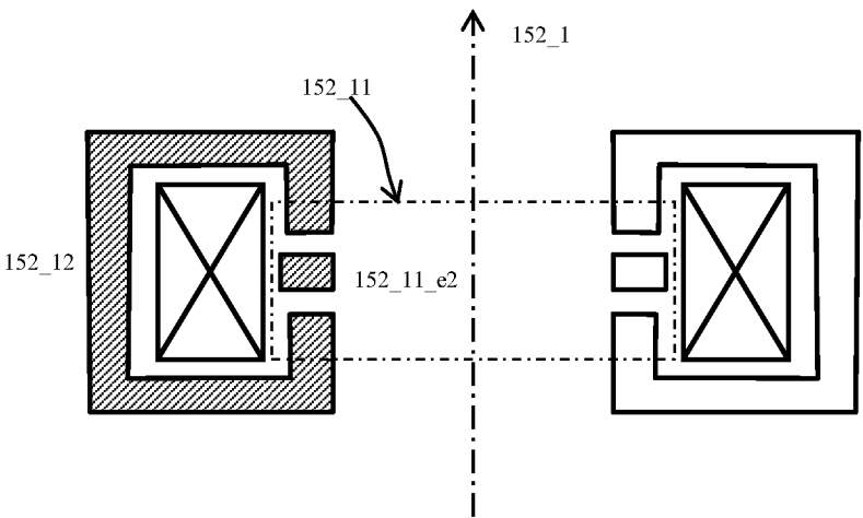
Figure 6C (Invention)
