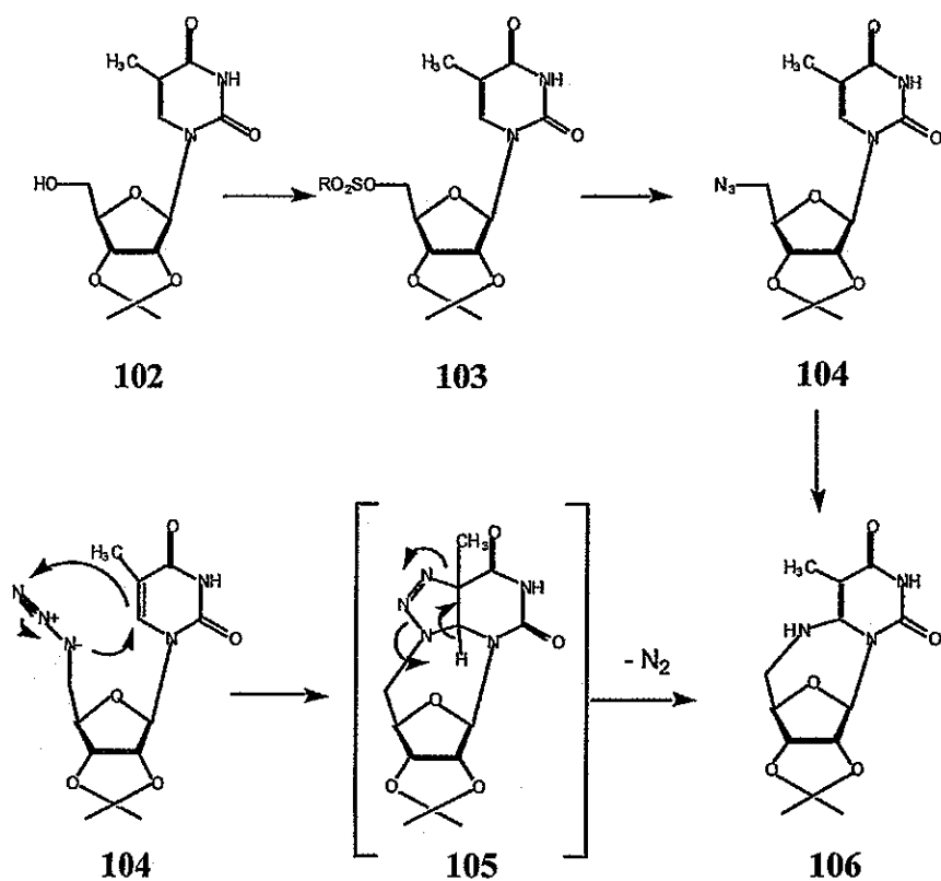
Scheme 15
