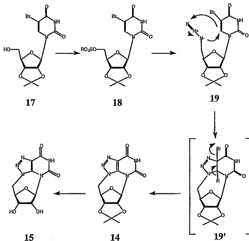
Scheme 2
