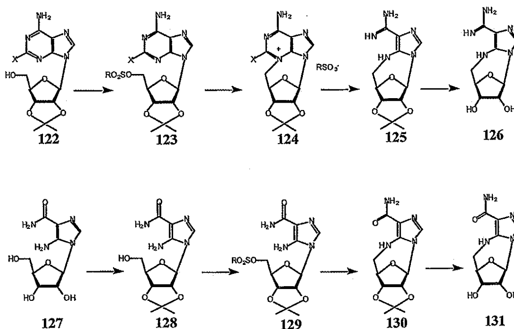
Scheme 20
