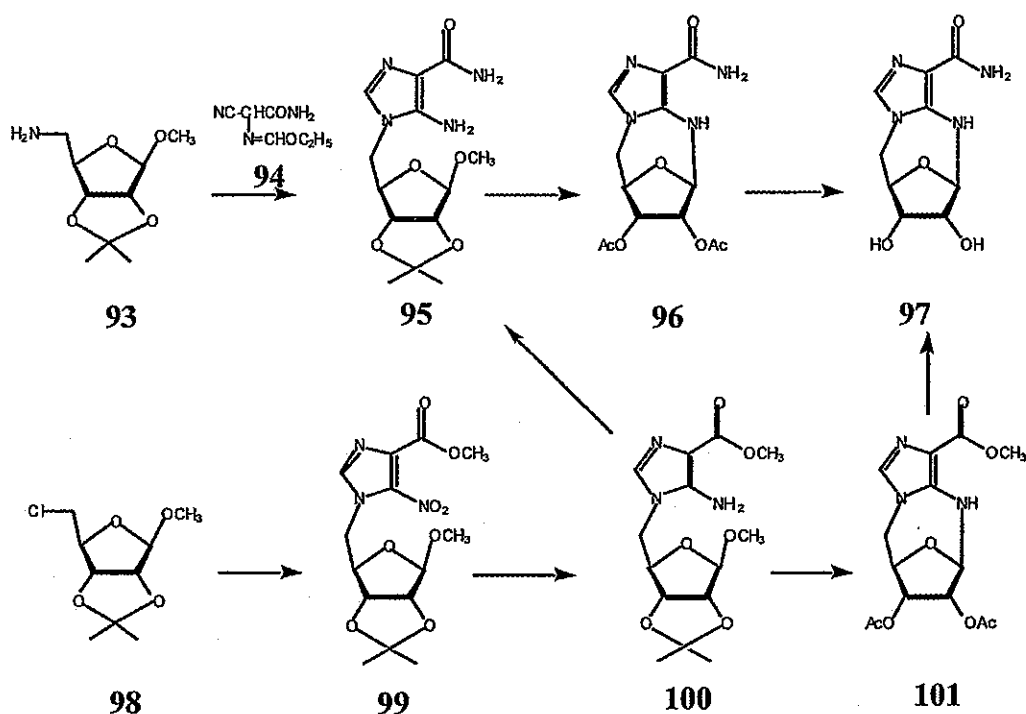
Scheme 14
