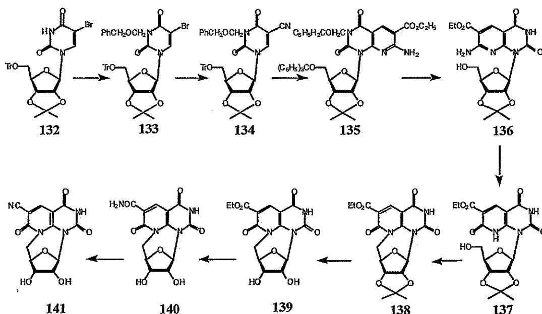
Scheme 21
