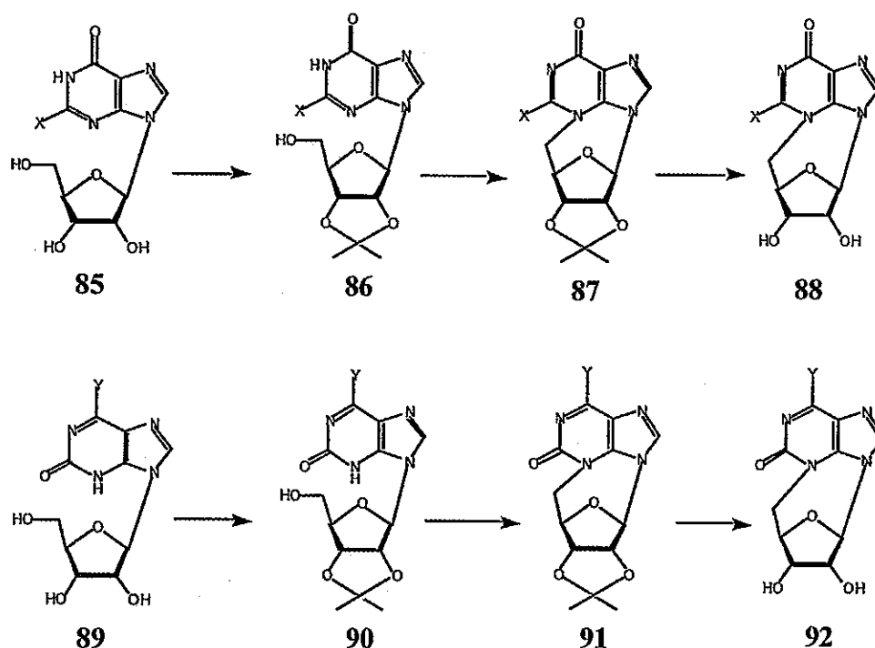
Scheme 13
