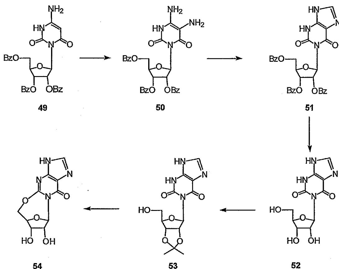
Scheme 7
