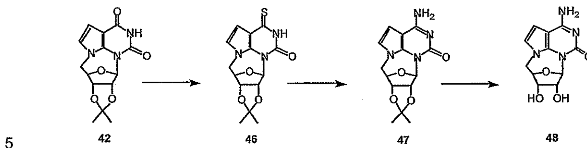
Scheme 6
