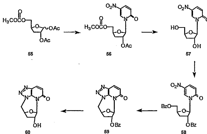
Scheme 8
