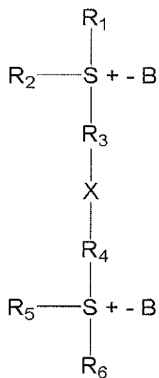
[Chemical Formula 15]
