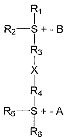
[Chemical Formula 1]
