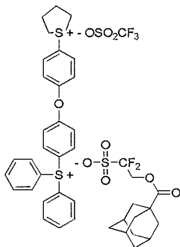
[Chemical Formula 5-11]
