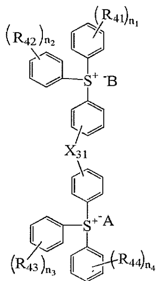
[Chemical Formula 4-2]
