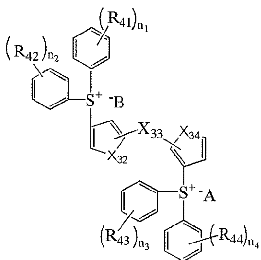
[Chemical Formula 4-5]
