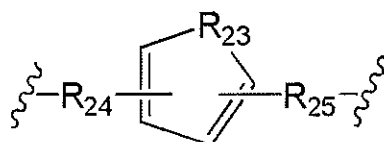
[Chemical Formula 2-2]
