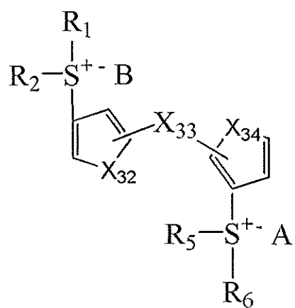
[Chemical Formula 3-3]
