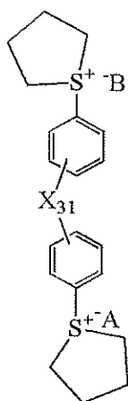
[Chemical Formula 4-4]
