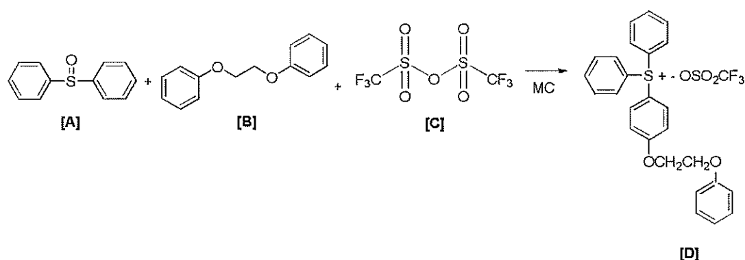
[Reaction Scheme 4]
