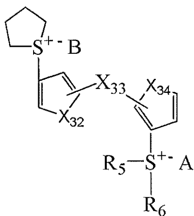
[Chemical Formula 3-3]
