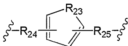
[Chemical Formula 2-2]
