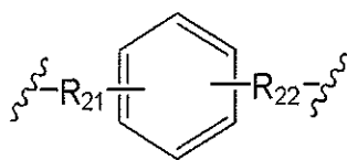
[Chemical Formula 2-2]
