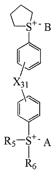
[Chemical Formula 3-2]
