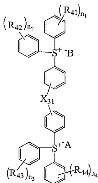
[Chemical Formula 4-2]
