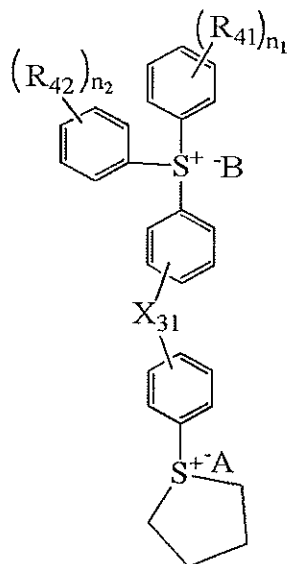
[Chemical Formula 4-3]
