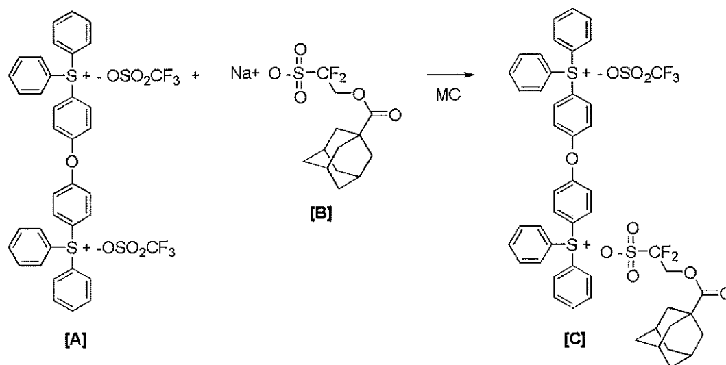
[Reaction Scheme 3]
