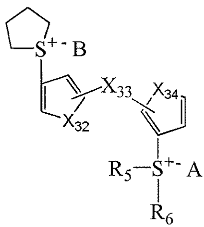
[Chemical Formula 3-3]
