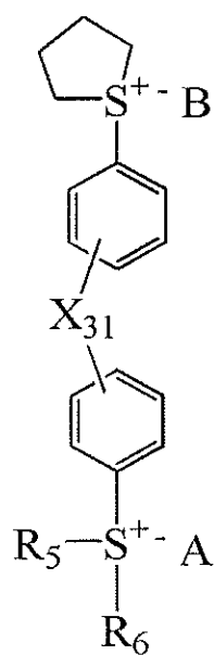
[Chemical Formula 3-2]
