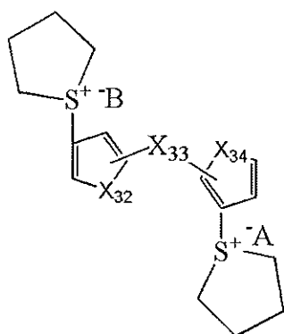
[Chemical Formula 4-6]
