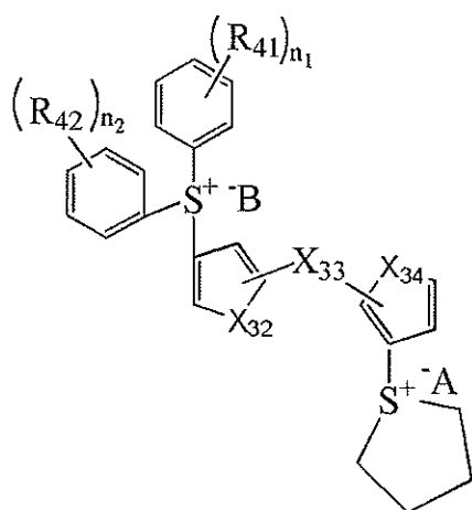
[Chemical Formula 4-5]
