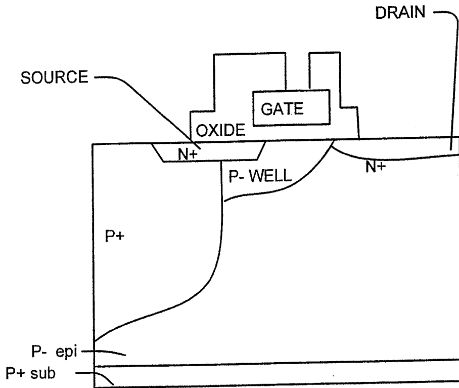
NON-OFFSET LDMOS FIGURE 8
