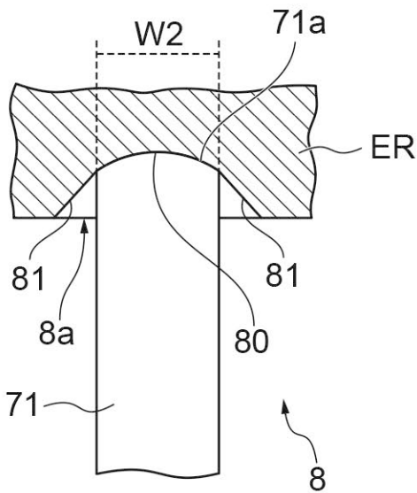
CROSS-SECTION A-A
