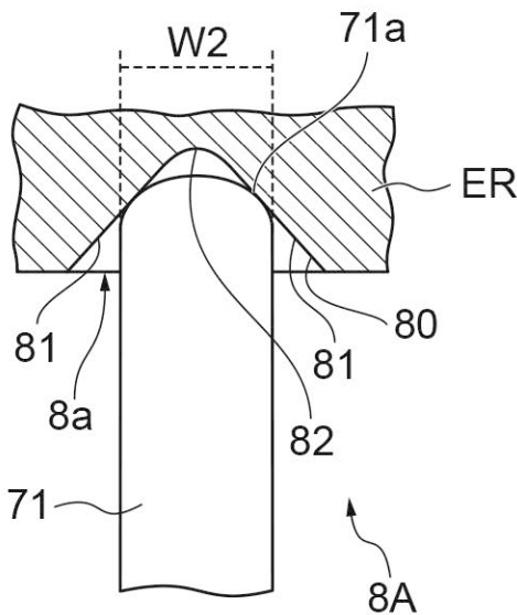
CROSS-SECTION A-A
