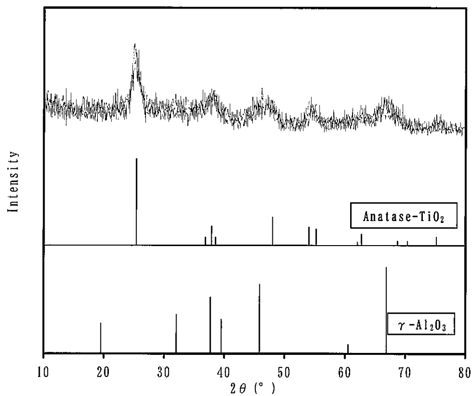
X-RAY DIFFRACTION PATTERN OF TITANIA-MIXED ALUMINA SUPPORT AT-14
