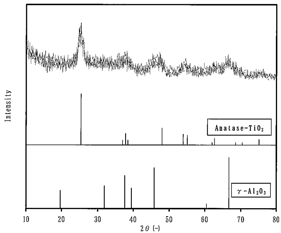
X-RAY ANALYSIS PATTERN OF TITANIA-COATED ALUMINA SUPPORT AT-13
