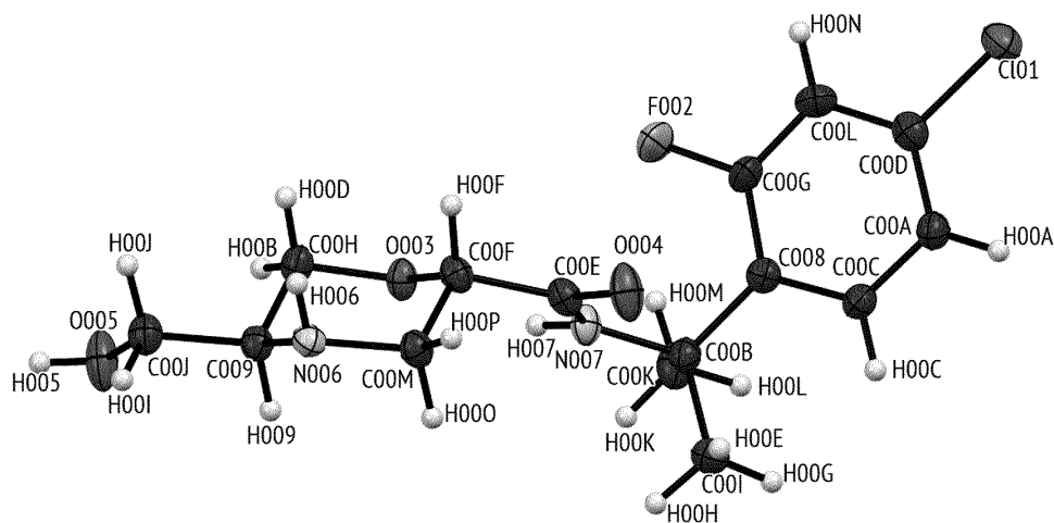
Figure 1B, Chemical structure of Reference Example trans-15 ( 2S,5S -configuration; trans ) as determined by single-crystal X-Ray analysis:
