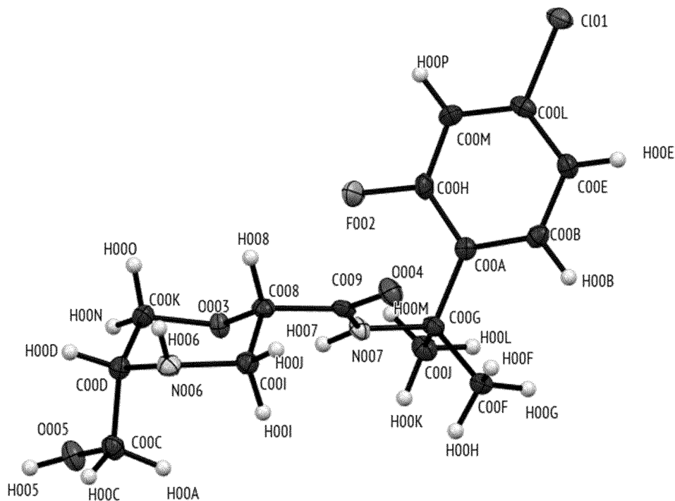
Figure 1A, Chemical structure of Example 15 ( 2S,5R -configuration; cis ) as determined by single-crystal X-Ray analysis:
