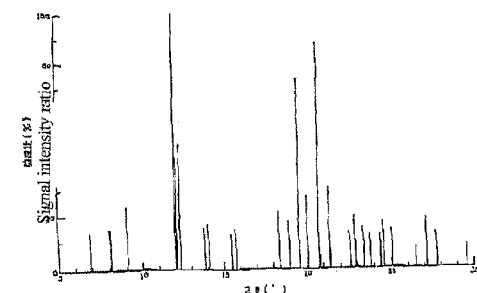
Powder X-ray Diffraction Pattern of form I.
