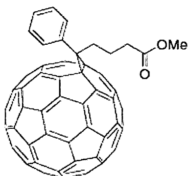
\text{C}_{60}\text{PCBM}
