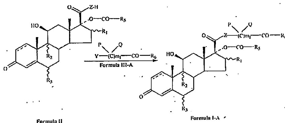
Scheme-II
