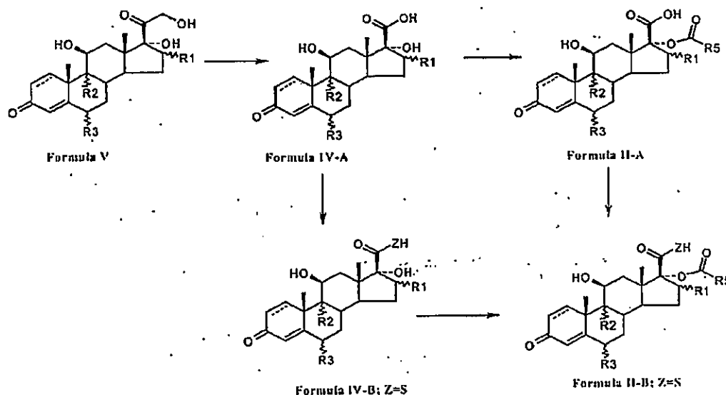
Scheme-III
