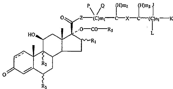
Formula I-B
