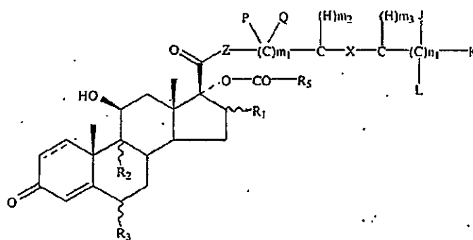
Formula I-B
