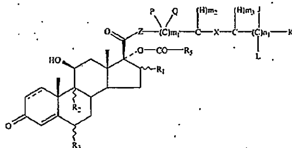
Formula I-B
