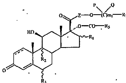
Formula I-C
