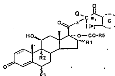
Formula I-A-2
