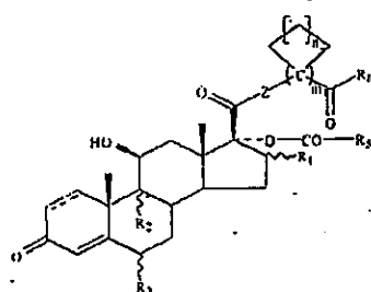
Formula I-A-1
