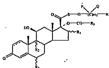
Formula I-C
