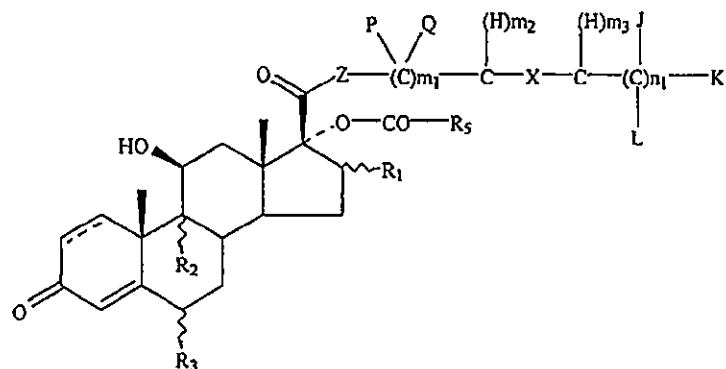
Formula I-B
