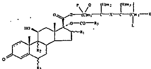
Formula I-B
