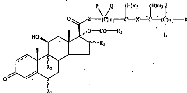
Formula I-B
