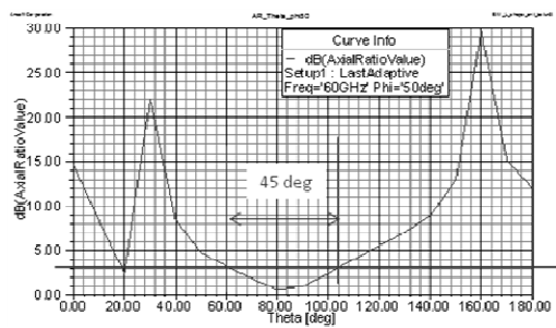
Axial ratio (angle)
