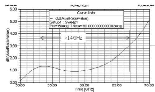
Axial ratio (Frequency)
