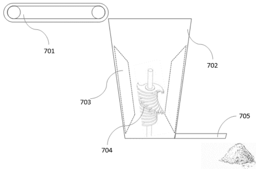
Figure 7 shows the granulation chamber for plastic & thin film, paper, cardboard, and organic waste.
