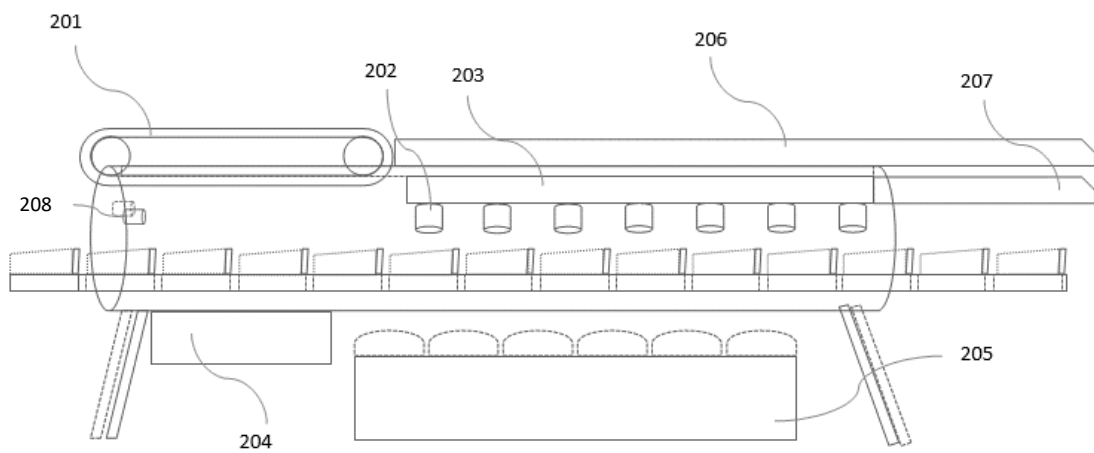
Figure 2 shows the sorting of ferrous metals and non-ferrous metals.
