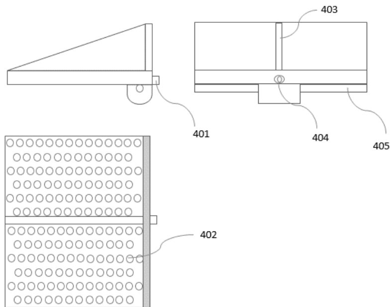
Figure 4 shows the detailed view of the conveyor tray in Figure 1, 2 and 3.
