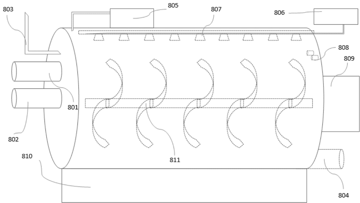
Figure 8 shows the acetogenic chamber.
