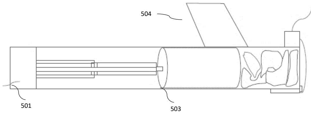
Figure 5B shows the thin film waste and the low density or low weight plastics being compressed.
