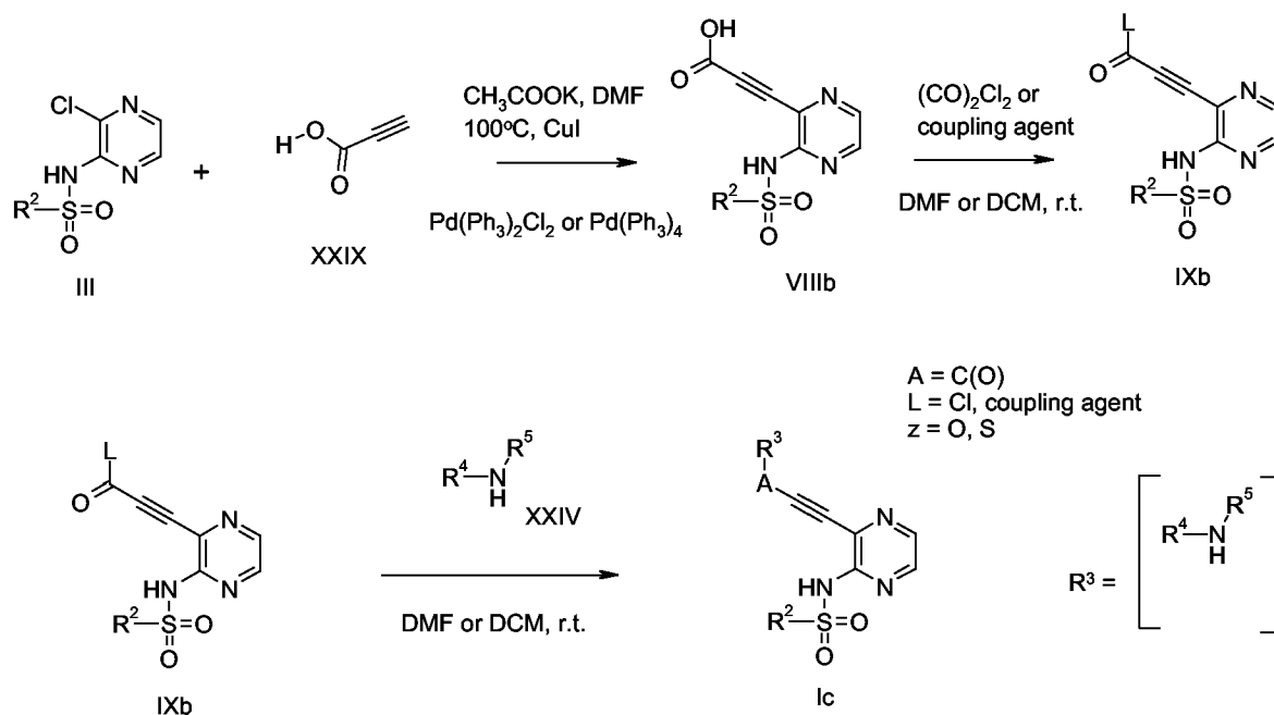
Scheme 9
