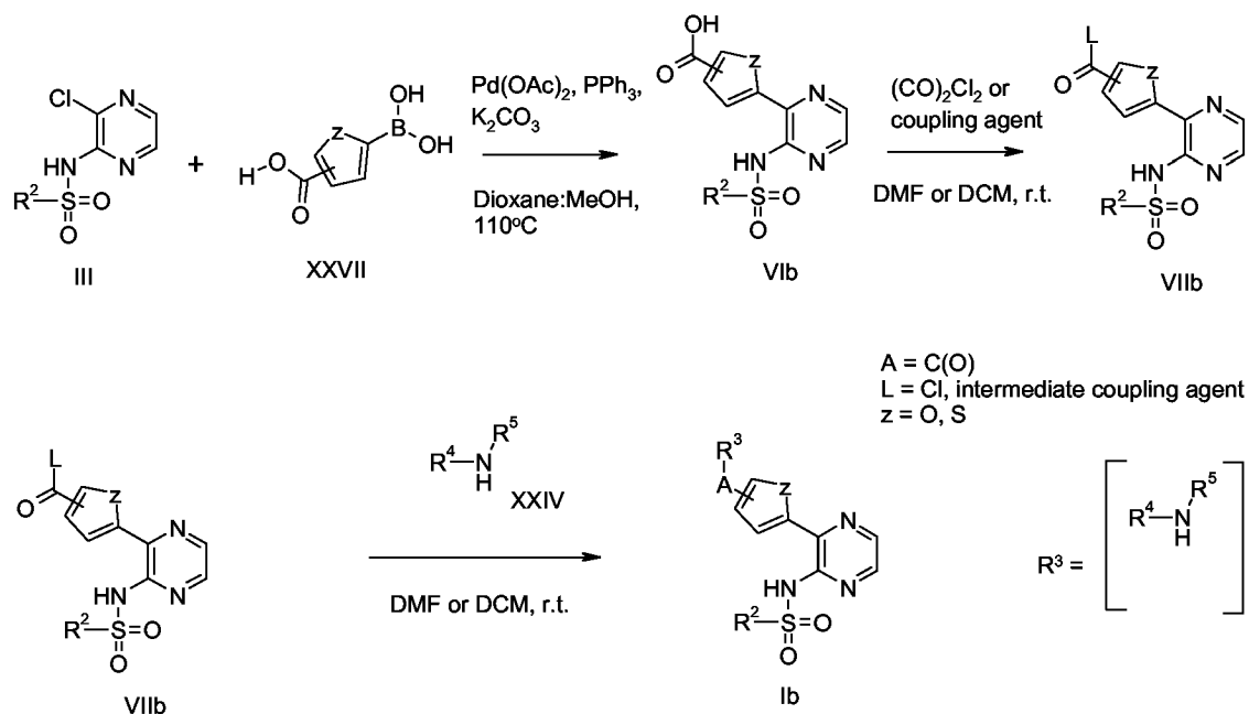
Scheme 7
