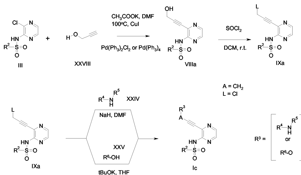
15 Scheme 8
