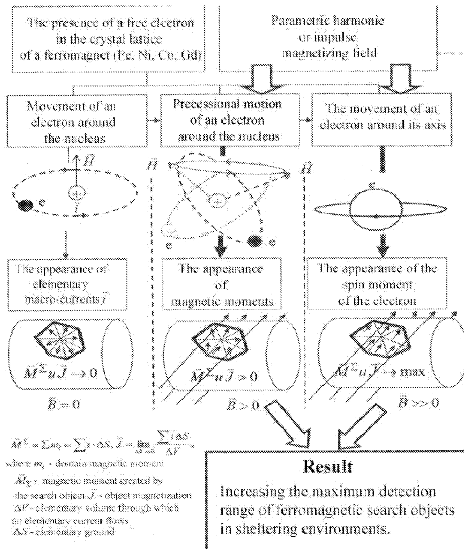
Fig. 3 - Causal structure of the process of parametric magnetization of search objects
